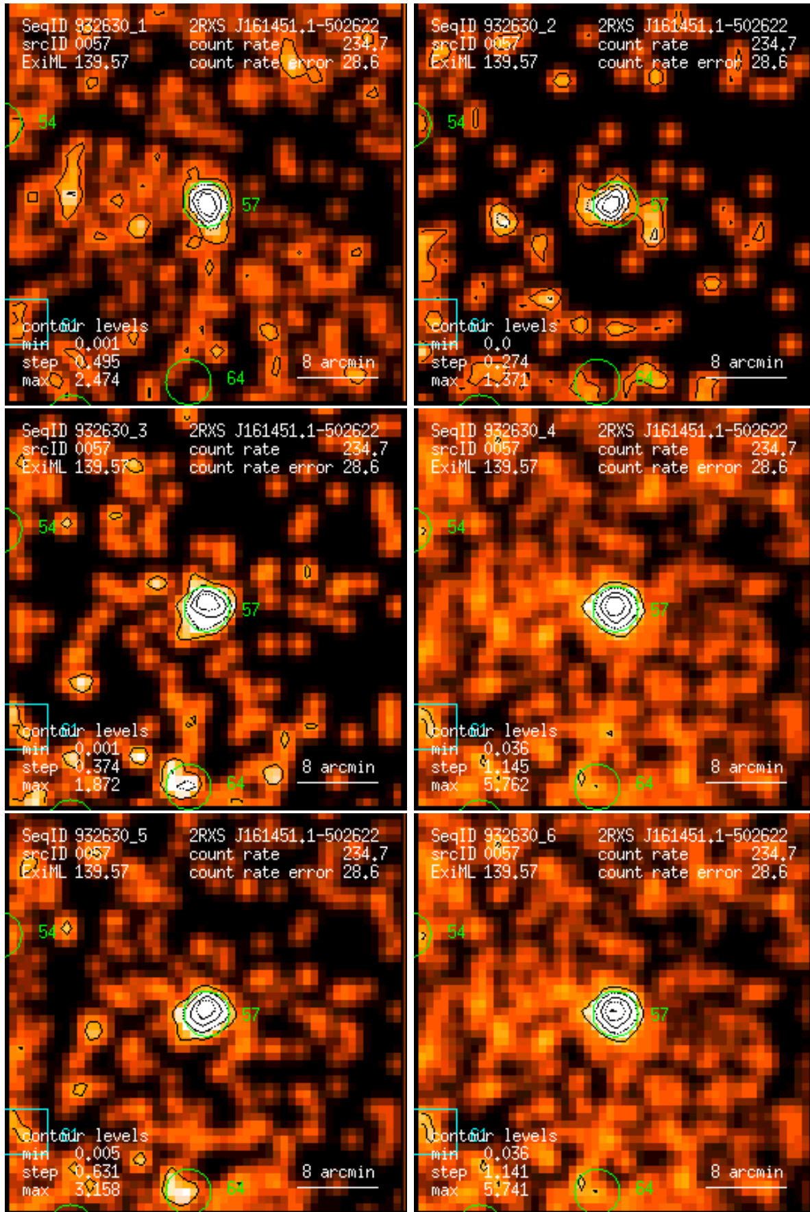
Figure 57: RASS 932630: detection 0057: band rate images, Gaussian filter: (1) PSPC channels 11 – 41, (2) 52 – 90, (3) 91 – 201, (4) 11 – 235, (5) 52 – 201, (6) 11 – 201. Broad band rates in counts/ks. Band rate contour levels in counts/ks/arcmin 2 .
