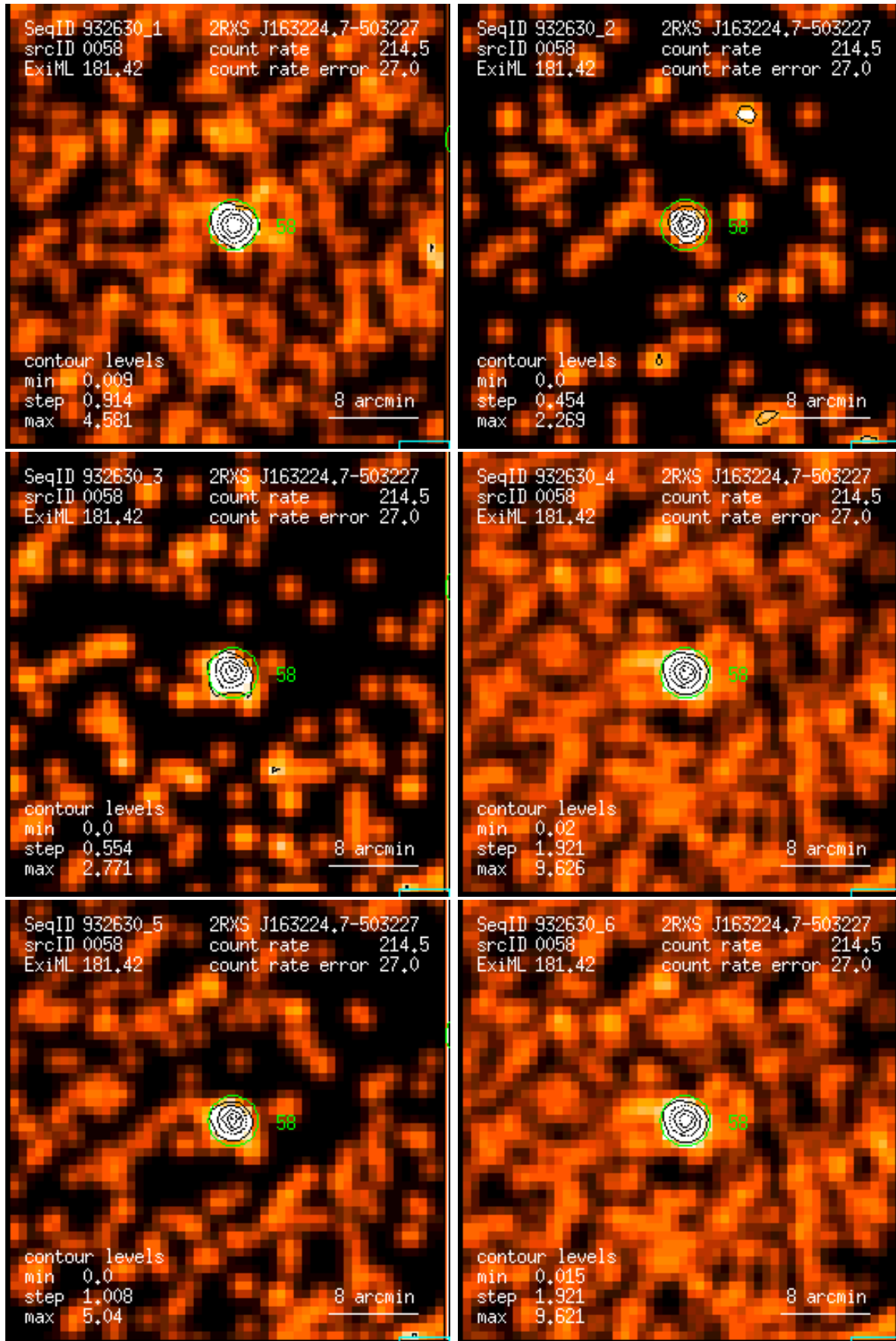
Figure 58: RASS 932630: detection 0058: band rate images, Gaussian filter: (1) PSPC channels 11 – 41, (2) 52 – 90, (3) 91 – 201, (4) 11 – 235, (5) 52 – 201, (6) 11 – 201. Broad band rates in counts/ks. Band rate contour levels in counts/ks/arcmin 2 .
