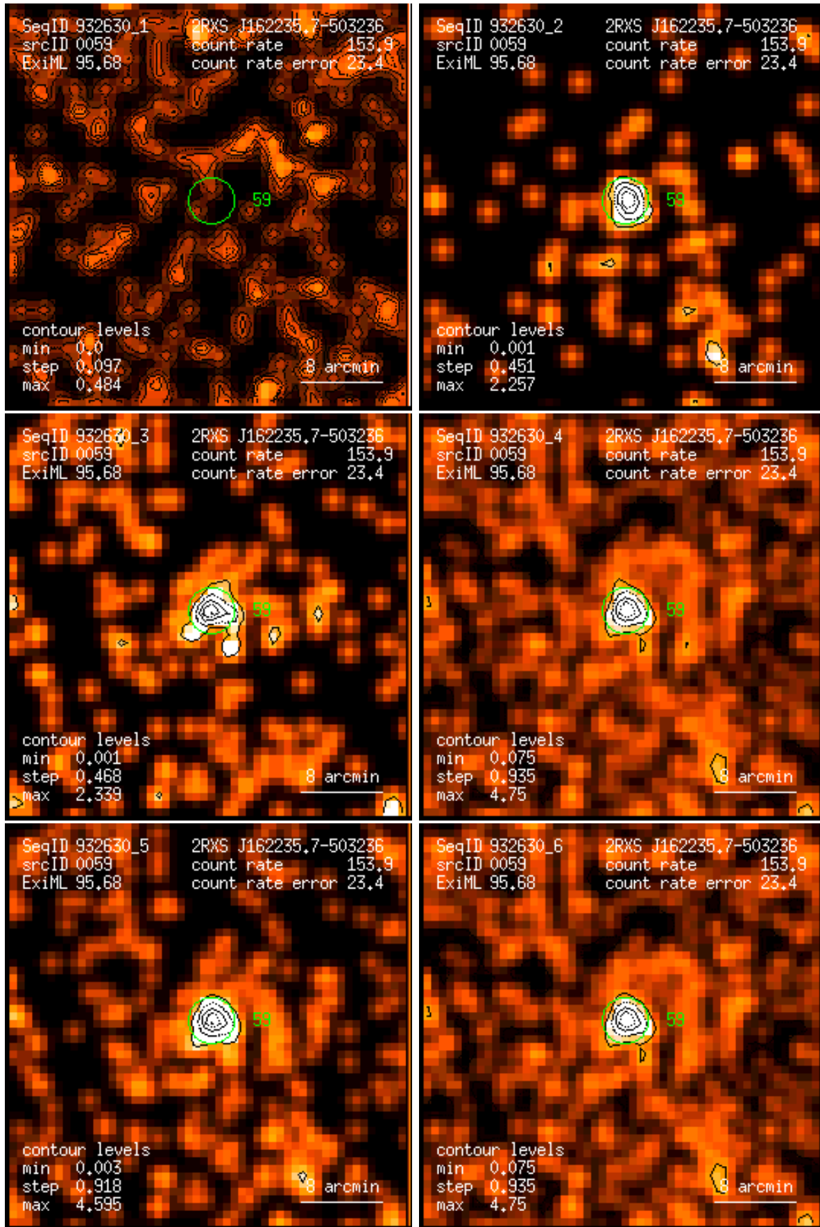
Figure 59: RASS 932630: detection 0059: band rate images, Gaussian filter: (1) PSPC channels 11 – 41, (2) 52 – 90, (3) 91 – 201, (4) 11 – 235, (5) 52 – 201, (6) 11 – 201. Broad band rates in counts/ks. Band rate contour levels in counts/ks/arcmin 2 .
