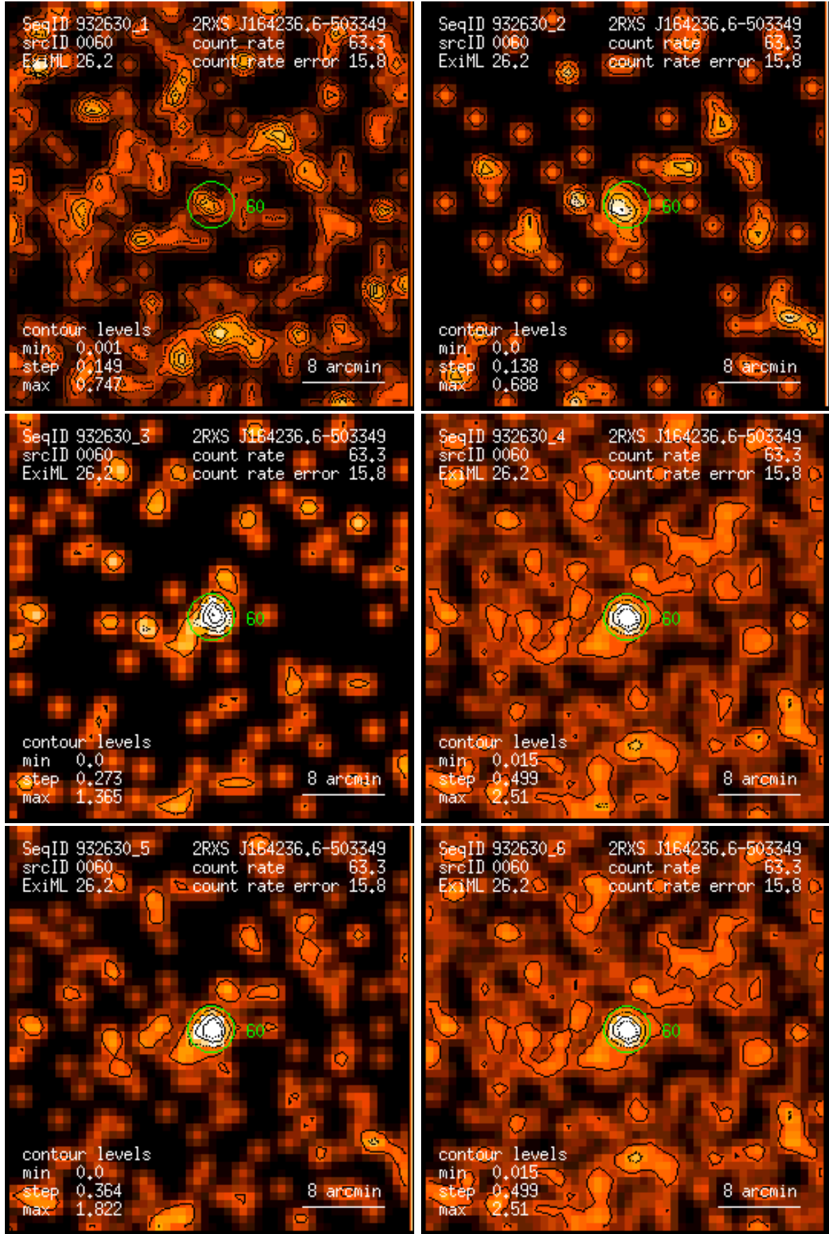
Figure 60: RASS 932630: detection 0060: band rate images, Gaussian filter: (1) PSPC channels 11 – 41, (2) 52 – 90, (3) 91 – 201, (4) 11 – 235, (5) 52 – 201, (6) 11 – 201. Broad band rates in counts/ks. Band rate contour levels in counts/ks/arcmin 2 .
