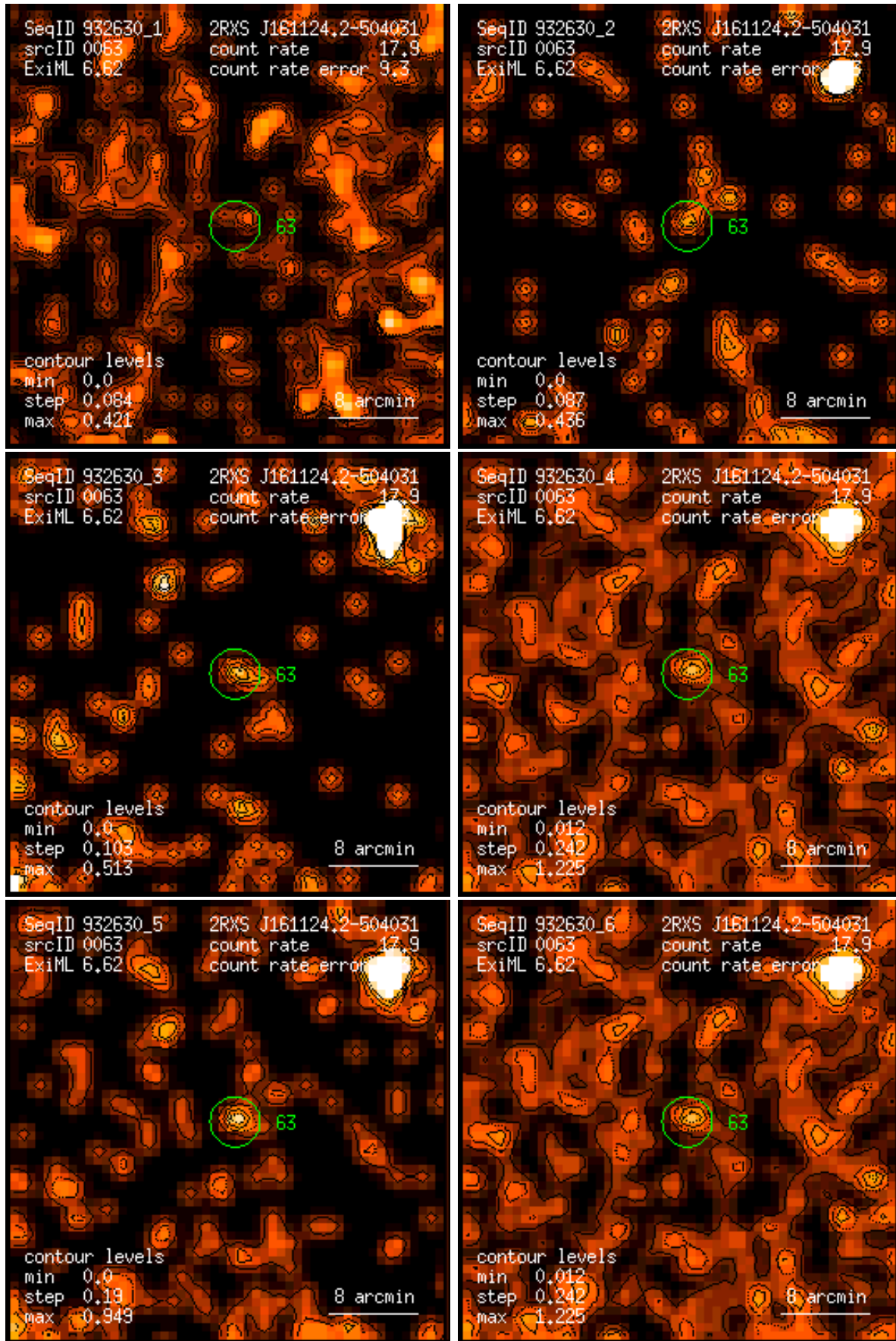
Figure 63: RASS 932630: detection 0063: band rate images, Gaussian filter: (1) PSPC channels 11 – 41, (2) 52 – 90, (3) 91 – 201, (4) 11 – 235, (5) 52 – 201, (6) 11 – 201. Broad band rates in counts/ks. Band rate contour levels in counts/ks/arcmin 2 .
