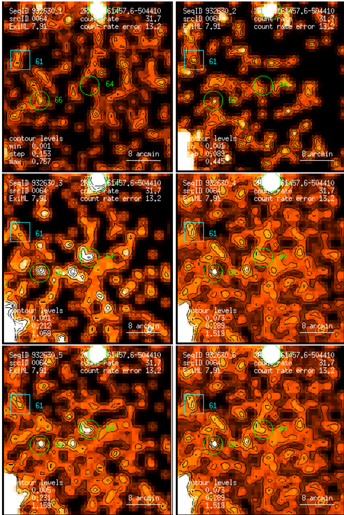
Figure 64: RASS 932630: detection 0064: band rate images, Gaussian filter: (1) PSPC channels 11 – 41, (2) 52 – 90, (3) 91 – 201, (4) 11 – 235, (5) 52 – 201, (6) 11 – 201. Broad band rates in counts/ks. Band rate contour levels in counts/ks/arcmin 2 .
