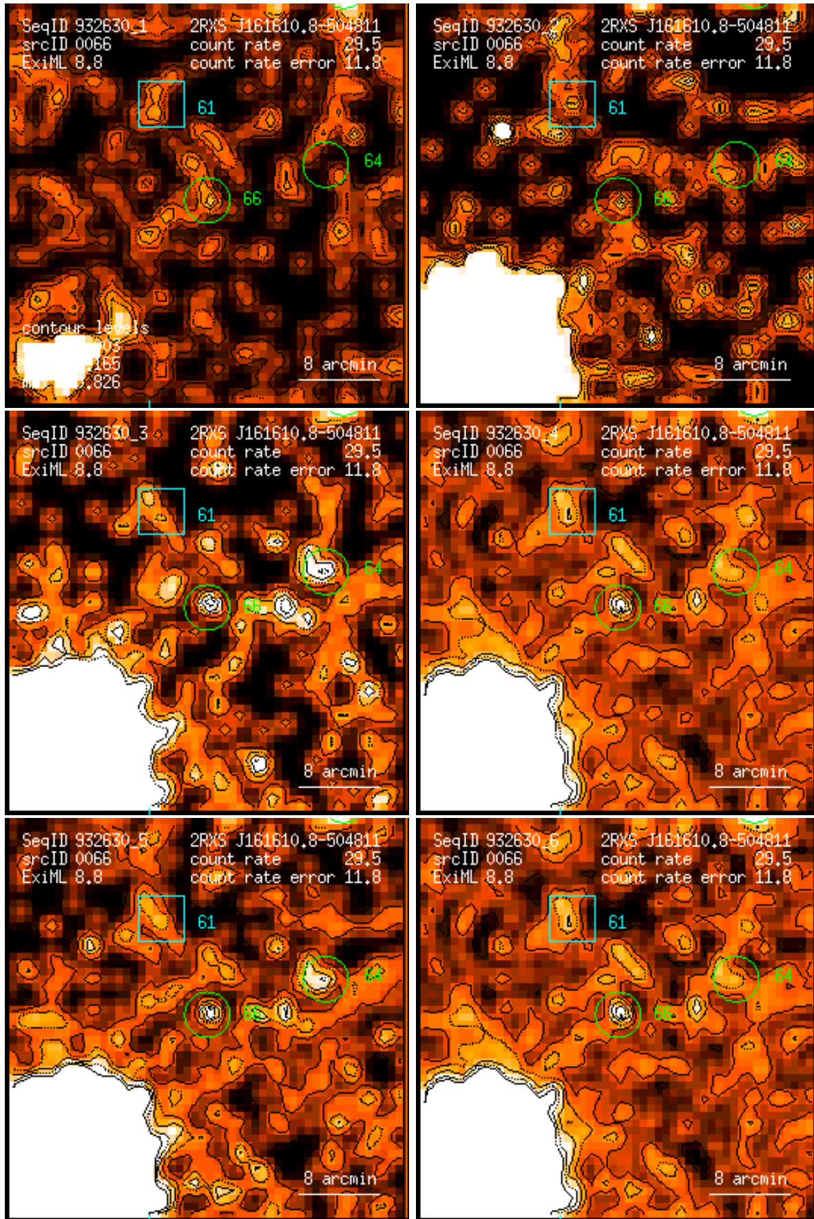
Figure 66: RASS 932630: detection 0066: band rate images, Gaussian filter: (1) PSPC channels 11 – 41, (2) 52 – 90, (3) 91 – 201, (4) 11 – 235, (5) 52 – 201, (6) 11 – 201. Broad band rates in counts/ks. Band rate contour levels in counts/ks/arcmin 2 .
