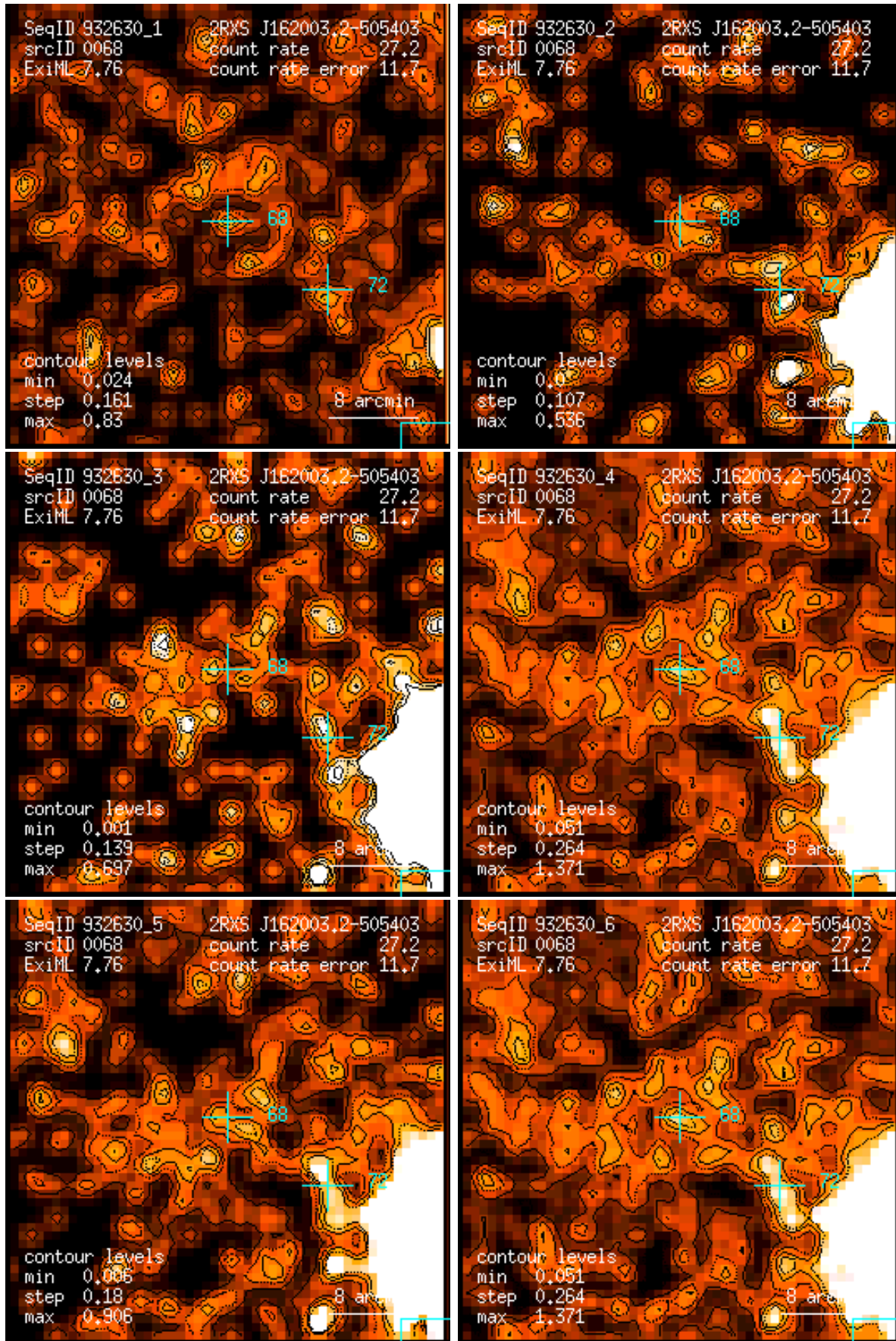
Figure 68: RASS 932630: detection 0068: band rate images, Gaussian filter: (1) PSPC channels 11 – 41, (2) 52 – 90, (3) 91 – 201, (4) 11 – 235, (5) 52 – 201, (6) 11 – 201. Broad band rates in counts/ks. Band rate contour levels in counts/ks/arcmin 2 .
