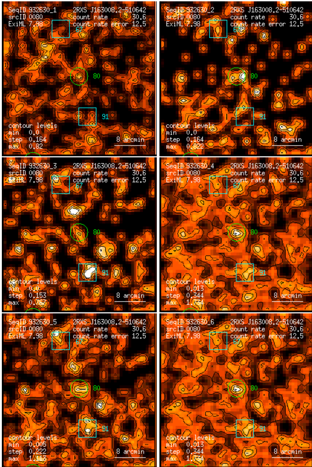
Figure 80: RASS 932630: detection 0080: band rate images, Gaussian filter: (1) PSPC channels 11 – 41, (2) 52 – 90, (3) 91 – 201, (4) 11 – 235, (5) 52 – 201, (6) 11 – 201. Broad band rates in counts/ks. Band rate contour levels in counts/ks/arcmin 2 .
