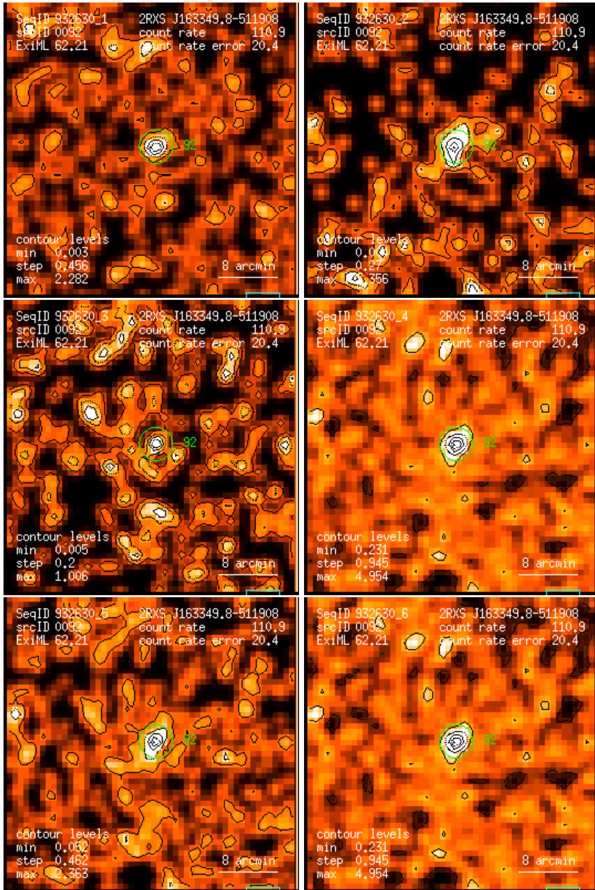
Figure 92: RASS 932630: detection 0092: band rate images, Gaussian filter: (1) PSPC channels 11 – 41, (2) 52 – 90, (3) 91 – 201, (4) 11 – 235, (5) 52 – 201, (6) 11 – 201. Broad band rates in counts/ks. Band rate contour levels in counts/ks/arcmin 2 .
