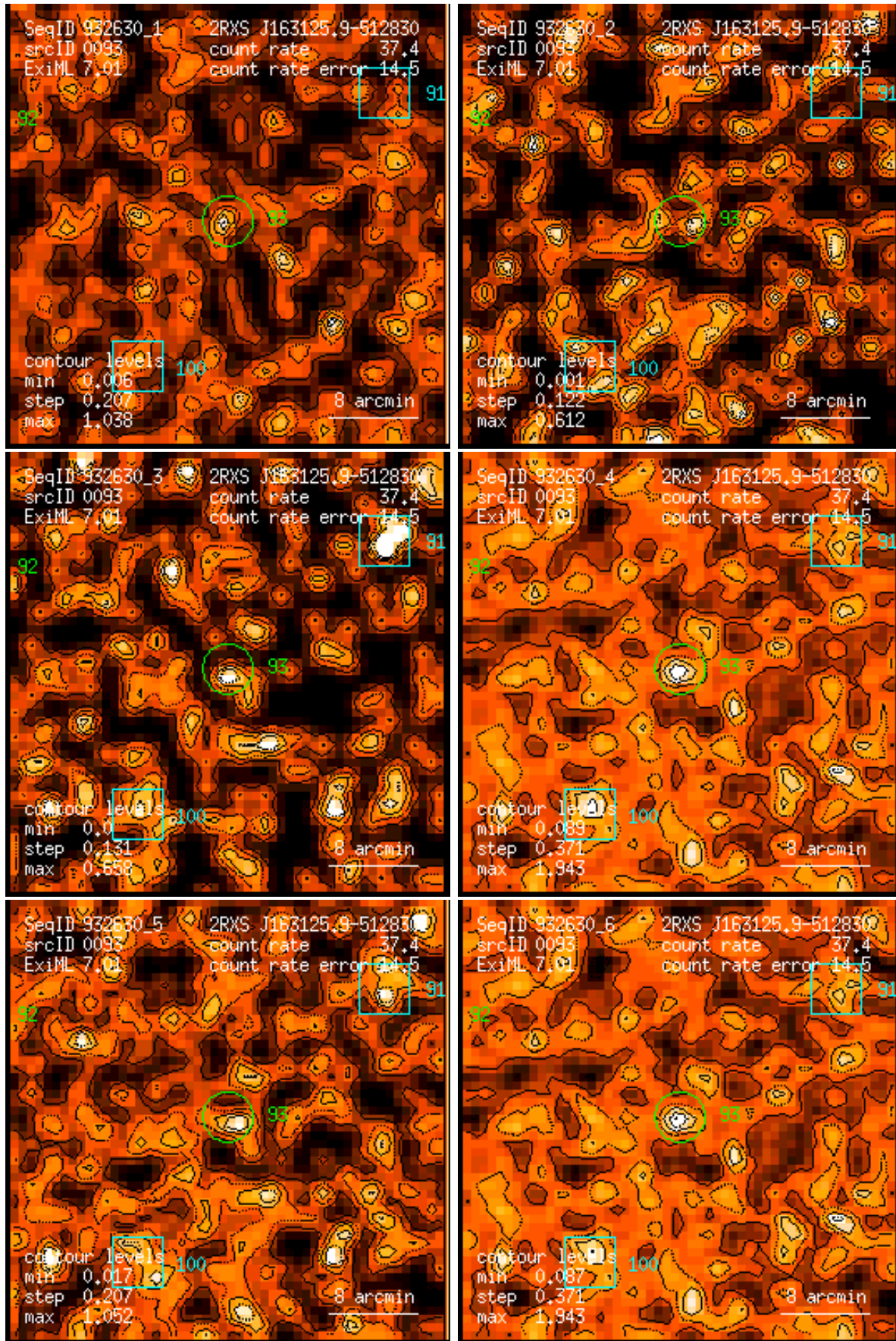
Figure 93: RASS 932630: detection 0093: band rate images, Gaussian filter: (1) PSPC channels 11 – 41, (2) 52 – 90, (3) 91 – 201, (4) 11 – 235, (5) 52 – 201, (6) 11 – 201. Broad band rates in counts/ks. Band rate contour levels in counts/ks/arcmin 2 .
