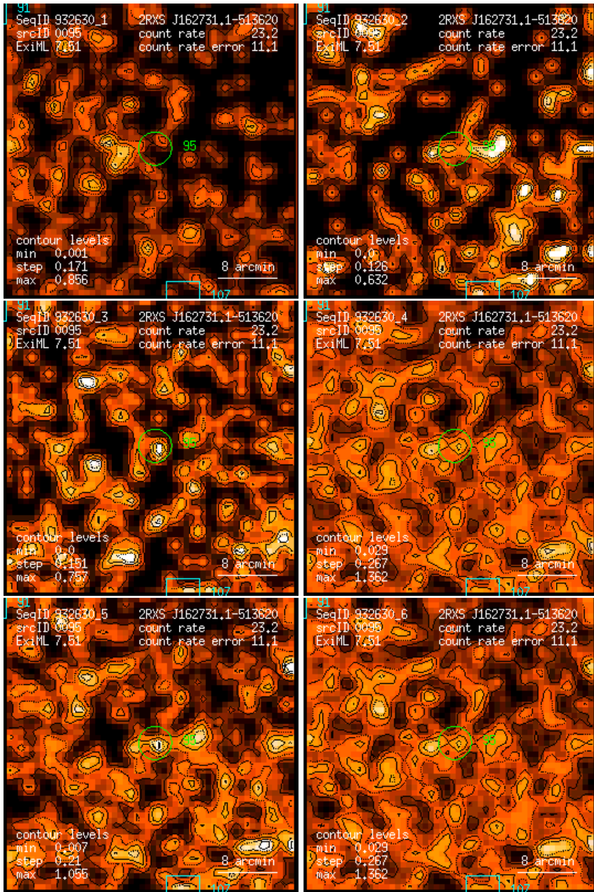
Figure 95: RASS 932630: detection 0095: band rate images, Gaussian filter: (1) PSPC channels 11 – 41, (2) 52 – 90, (3) 91 – 201, (4) 11 – 235, (5) 52 – 201, (6) 11 – 201. Broad band rates in counts/ks. Band rate contour levels in counts/ks/arcmin 2 .
