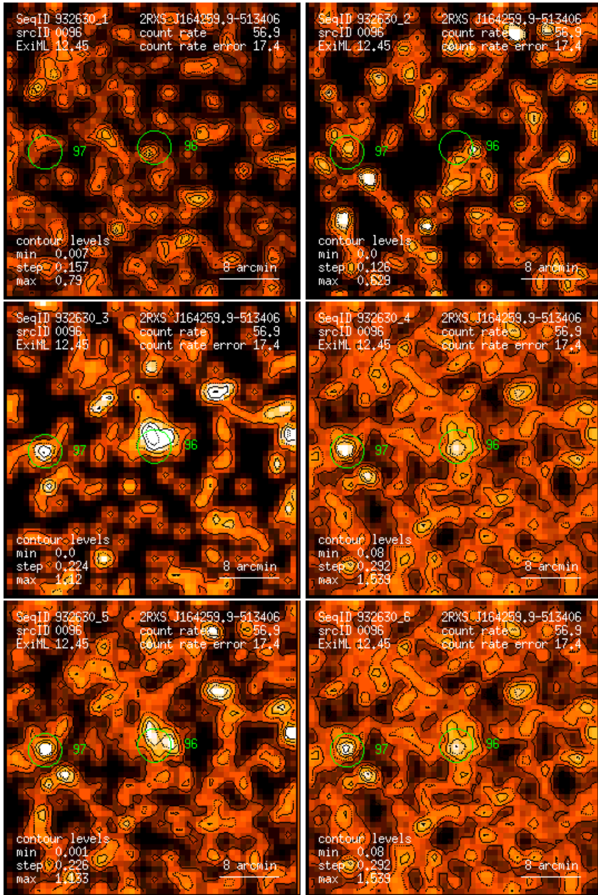
Figure 96: RASS 932630: detection 0096: band rate images, Gaussian filter: (1) PSPC channels 11 – 41, (2) 52 – 90, (3) 91 – 201, (4) 11 – 235, (5) 52 – 201, (6) 11 – 201. Broad band rates in counts/ks. Band rate contour levels in counts/ks/arcmin 2 .
