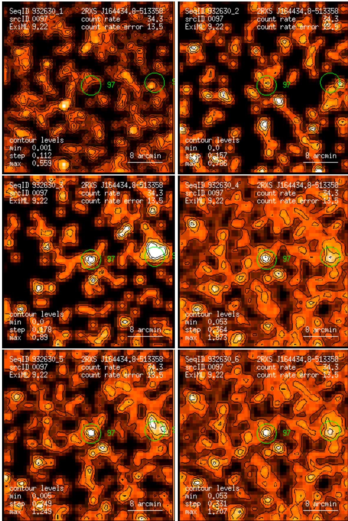
Figure 97: RASS 932630: detection 0097: band rate images, Gaussian filter: (1) PSPC channels 11 – 41, (2) 52 – 90, (3) 91 – 201, (4) 11 – 235, (5) 52 – 201, (6) 11 – 201. Broad band rates in counts/ks. Band rate contour levels in counts/ks/arcmin 2 .
