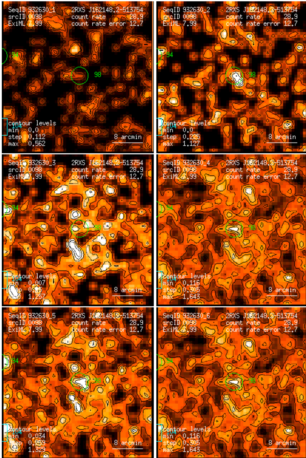
Figure 98: RASS 932630: detection 0098: band rate images, Gaussian filter: (1) PSPC channels 11 – 41, (2) 52 – 90, (3) 91 – 201, (4) 11 – 235, (5) 52 – 201, (6) 11 – 201. Broad band rates in counts/ks. Band rate contour levels in counts/ks/arcmin 2 .
