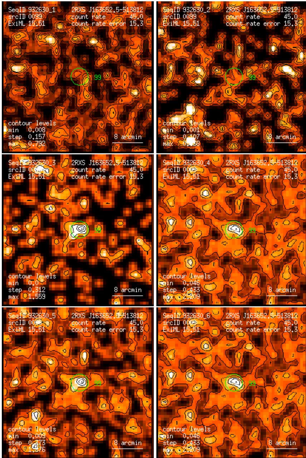
Figure 99: RASS 932630: detection 0099: band rate images, Gaussian filter: (1) PSPC channels 11 – 41, (2) 52 – 90, (3) 91 – 201, (4) 11 – 235, (5) 52 – 201, (6) 11 – 201. Broad band rates in counts/ks. Band rate contour levels in counts/ks/arcmin 2 .
