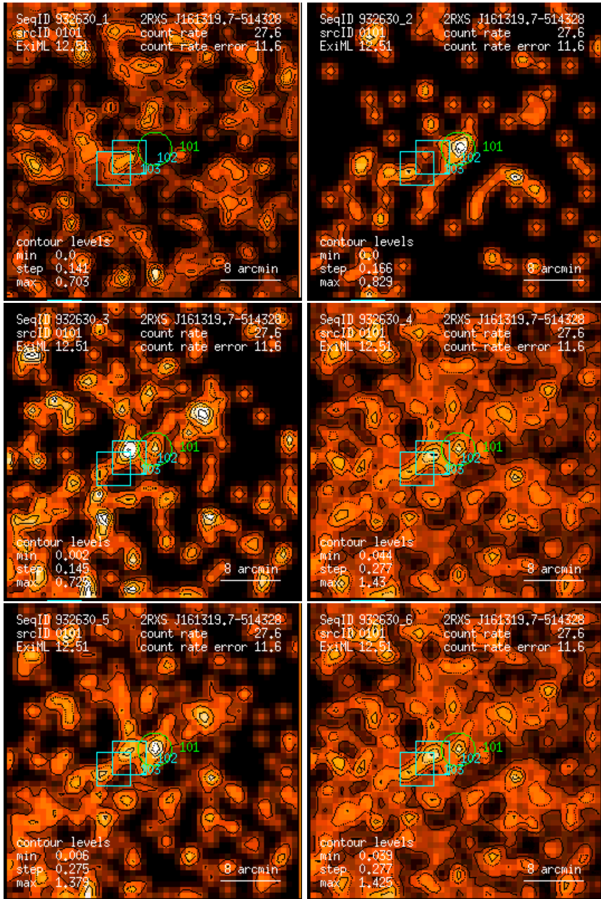
Figure 101: RASS 932630: detection 0101: band rate images, Gaussian filter: (1) PSPC channels 11 – 41, (2) 52 – 90, (3) 91 – 201, (4) 11 – 235, (5) 52 – 201, (6) 11 – 201. Broad band rates in counts/ks. Band rate contour levels in counts/ks/arcmin 2 .
