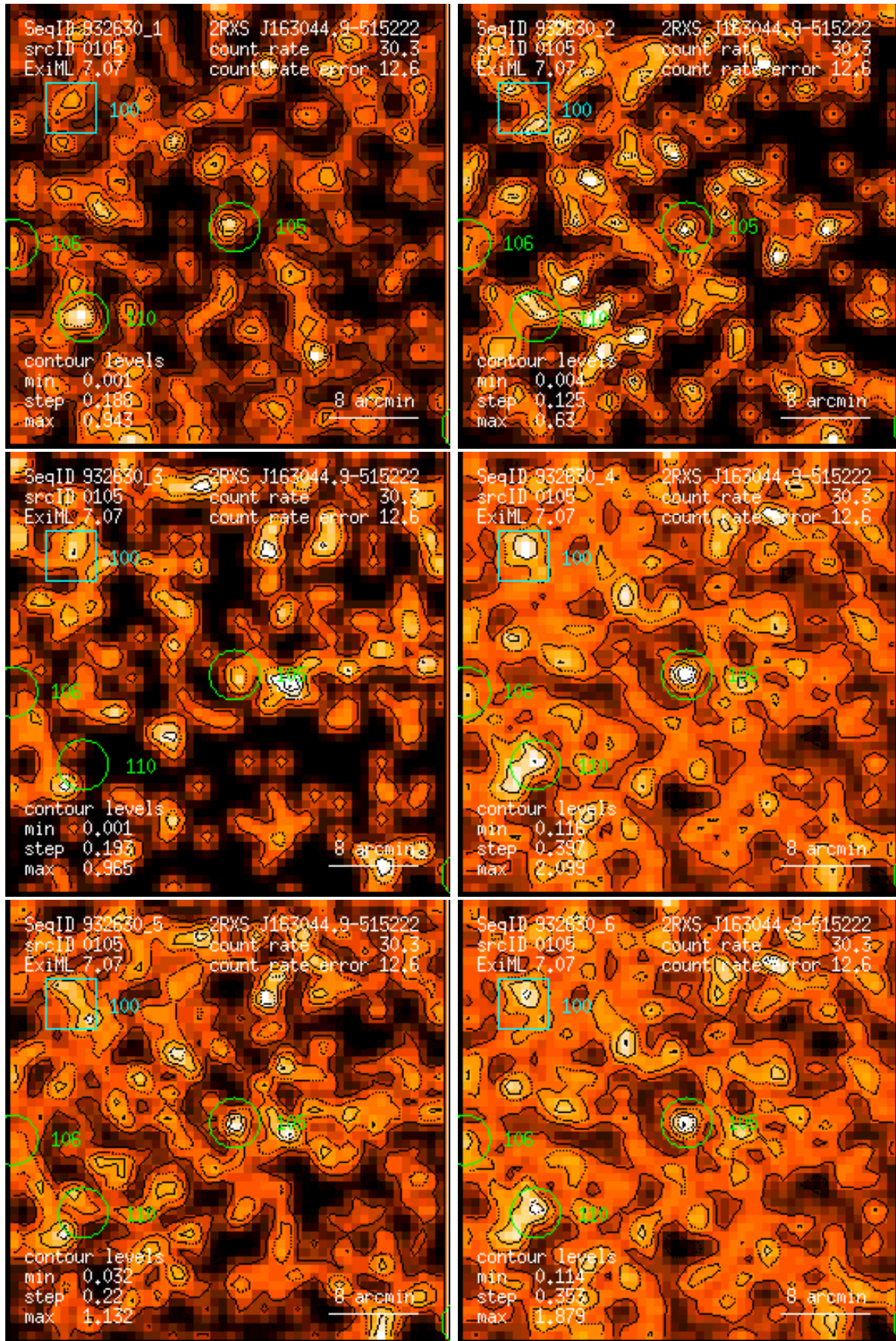
Figure 105: RASS 932630: detection 0105: band rate images, Gaussian filter: (1) PSPC channels 11 – 41, (2) 52 – 90, (3) 91 – 201, (4) 11 – 235, (5) 52 – 201, (6) 11 – 201. Broad band rates in counts/ks. Band rate contour levels in counts/ks/arcmin 2 .
