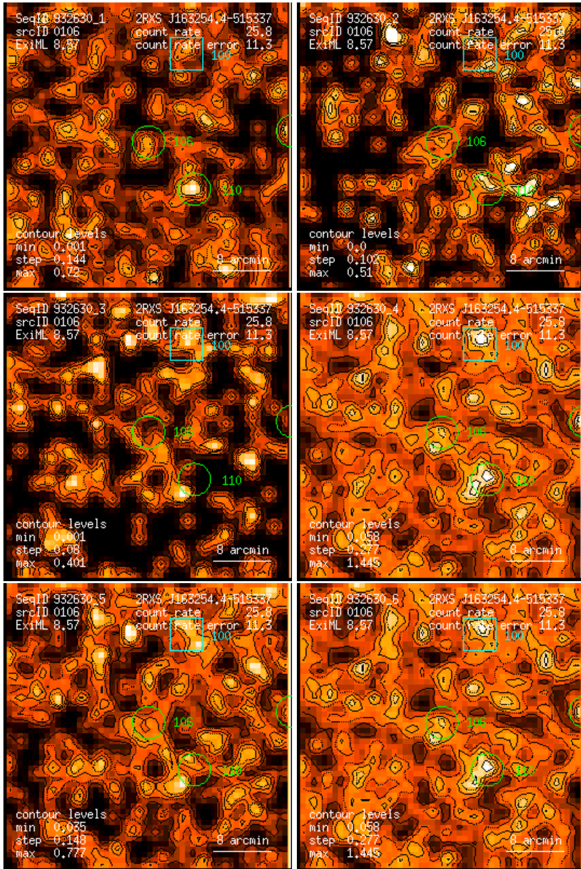
Figure 106: RASS 932630: detection 0106: band rate images, Gaussian filter: (1) PSPC channels 11 – 41, (2) 52 – 90, (3) 91 – 201, (4) 11 – 235, (5) 52 – 201, (6) 11 – 201. Broad band rates in counts/ks. Band rate contour levels in counts/ks/arcmin 2 .
