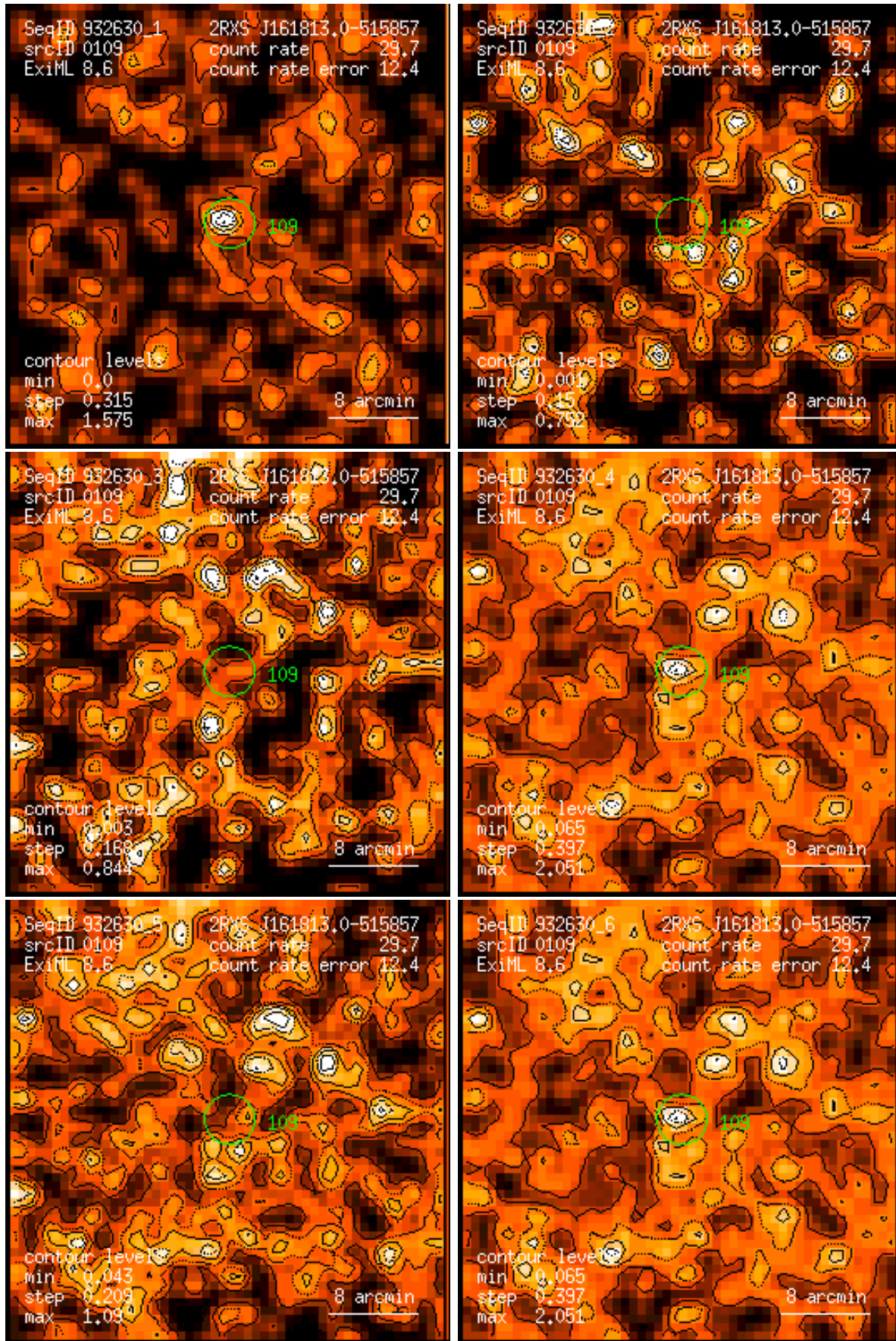
Figure 109: RASS 932630: detection 0109: band rate images, Gaussian filter: (1) PSPC channels 11 – 41, (2) 52 – 90, (3) 91 – 201, (4) 11 – 235, (5) 52 – 201, (6) 11 – 201. Broad band rates in counts/ks. Band rate contour levels in counts/ks/arcmin 2 .
