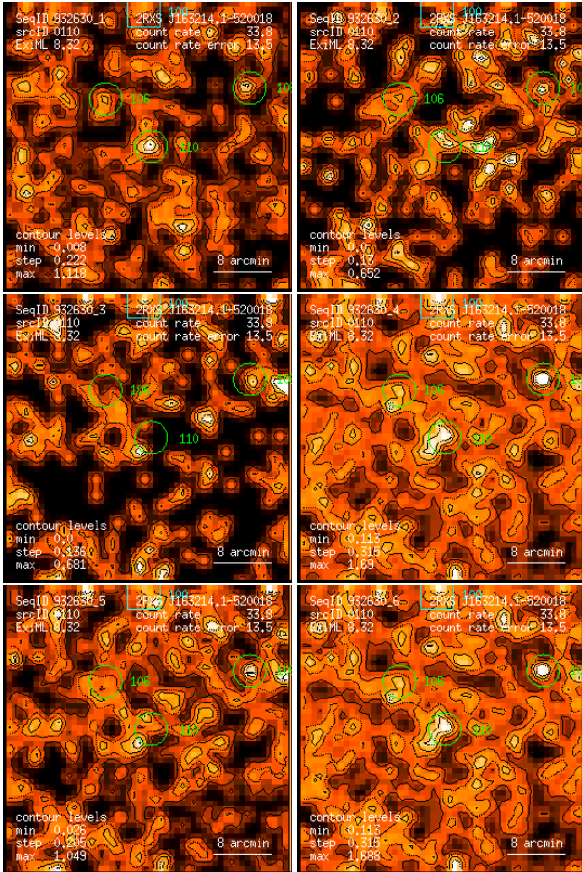
Figure 110: RASS 932630: detection 0110: band rate images, Gaussian filter: (1) PSPC channels 11 – 41, (2) 52 – 90, (3) 91 – 201, (4) 11 – 235, (5) 52 – 201, (6) 11 – 201. Broad band rates in counts/ks. Band rate contour levels in counts/ks/arcmin 2 .
