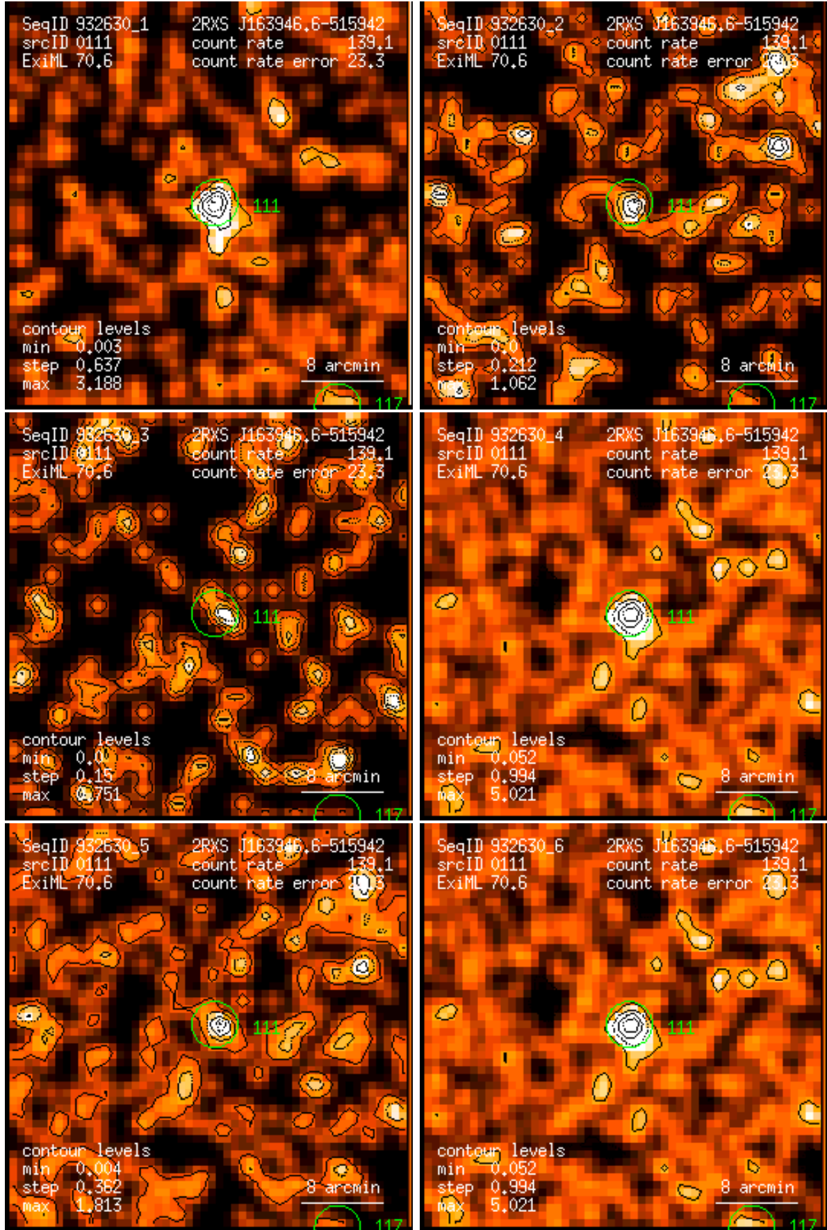
Figure 111: RASS 932630: detection 0111: band rate images, Gaussian filter: (1) PSPC channels 11 – 41, (2) 52 – 90, (3) 91 – 201, (4) 11 – 235, (5) 52 – 201, (6) 11 – 201. Broad band rates in counts/ks. Band rate contour levels in counts/ks/arcmin 2 .
