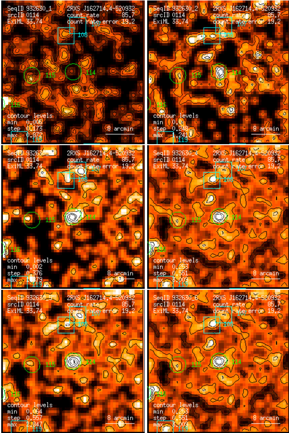
Figure 114: RASS 932630: detection 0114: band rate images, Gaussian filter: (1) PSPC channels 11 – 41, (2) 52 – 90, (3) 91 – 201, (4) 11 – 235, (5) 52 – 201, (6) 11 – 201. Broad band rates in counts/ks. Band rate contour levels in counts/ks/arcmin 2 .
