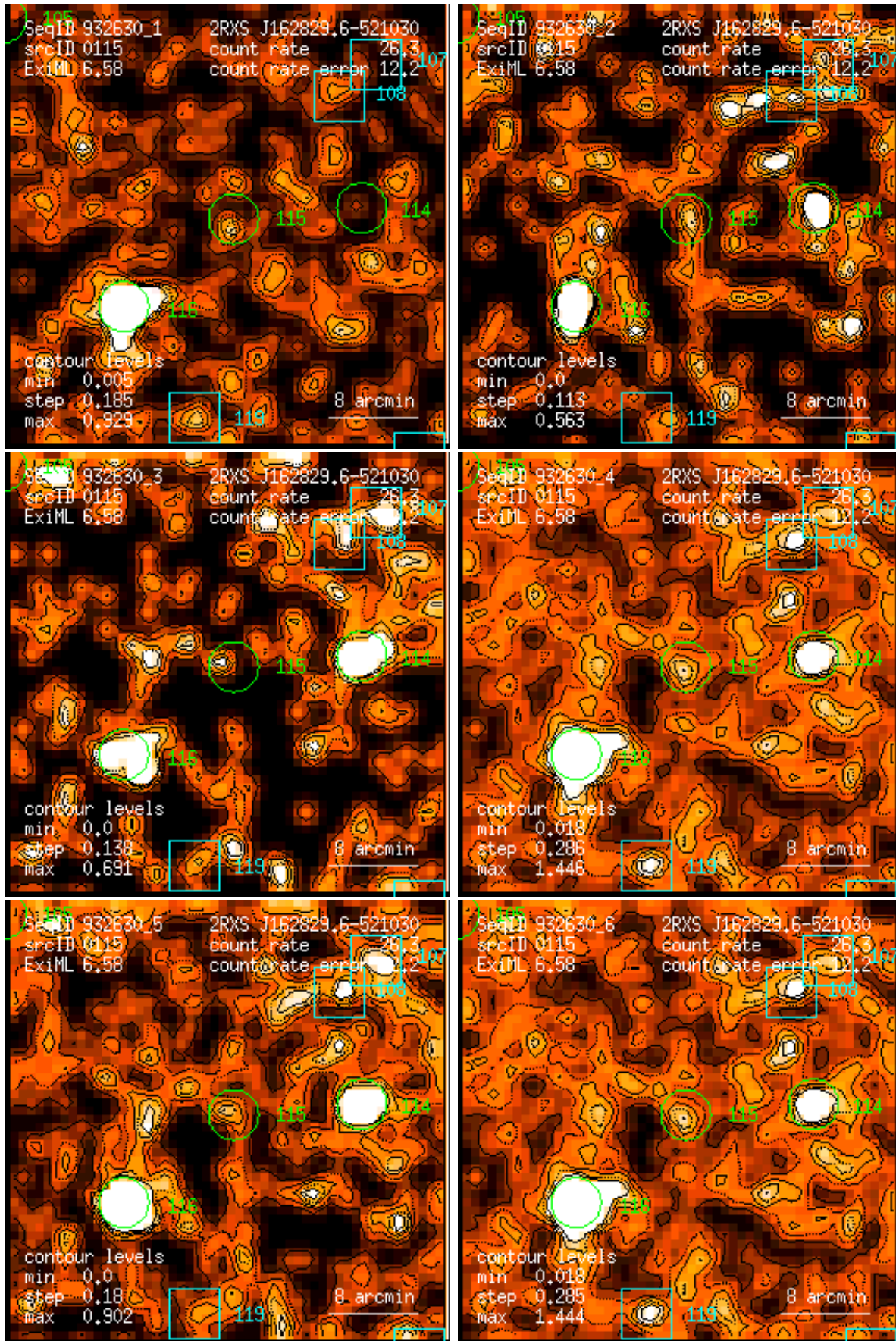
Figure 115: RASS 932630: detection 0115: band rate images, Gaussian filter: (1) PSPC channels 11 – 41, (2) 52 – 90, (3) 91 – 201, (4) 11 – 235, (5) 52 – 201, (6) 11 – 201. Broad band rates in counts/ks. Band rate contour levels in counts/ks/arcmin 2 .
