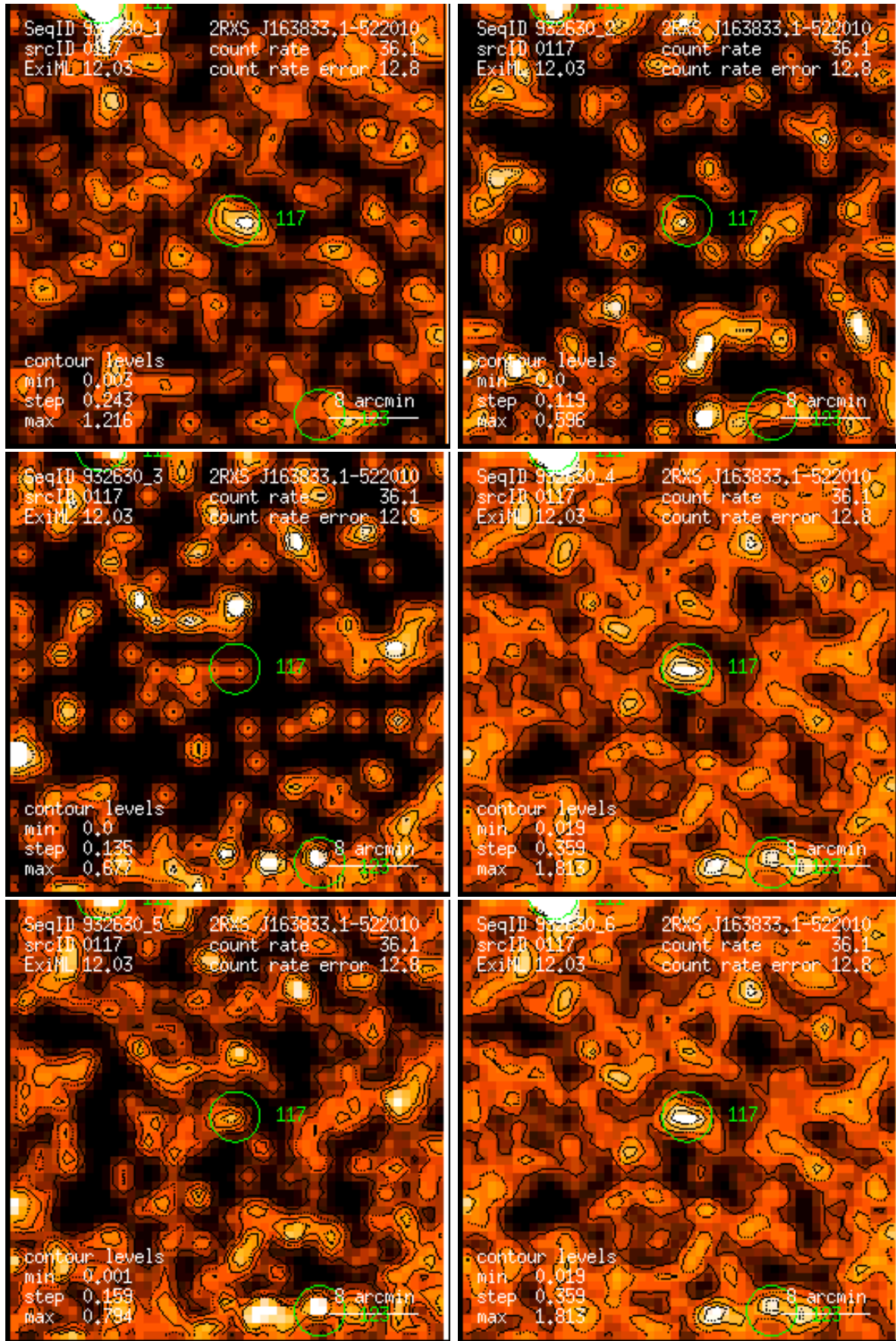
Figure 117: RASS 932630: detection 0117: band rate images, Gaussian filter: (1) PSPC channels 11 – 41, (2) 52 – 90, (3) 91 – 201, (4) 11 – 235, (5) 52 – 201, (6) 11 – 201. Broad band rates in counts/ks. Band rate contour levels in counts/ks/arcmin 2 .
