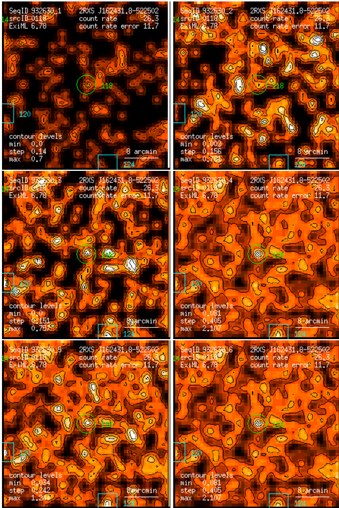
Figure 118: RASS 932630: detection 0118: band rate images, Gaussian filter: (1) PSPC channels 11 – 41, (2) 52 – 90, (3) 91 – 201, (4) 11 – 235, (5) 52 – 201, (6) 11 – 201. Broad band rates in counts/ks. Band rate contour levels in counts/ks/arcmin 2 .
