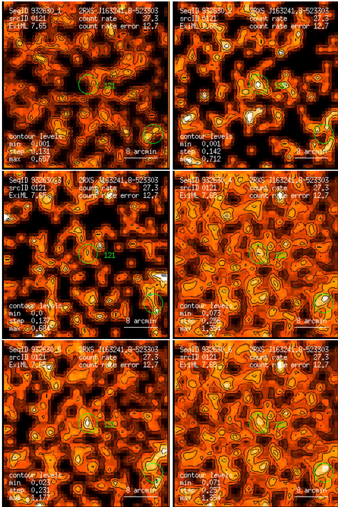
Figure 121: RASS 932630: detection 0121: band rate images, Gaussian filter: (1) PSPC channels 11 – 41, (2) 52 – 90, (3) 91 – 201, (4) 11 – 235, (5) 52 – 201, (6) 11 – 201. Broad band rates in counts/ks. Band rate contour levels in counts/ks/arcmin 2 .
