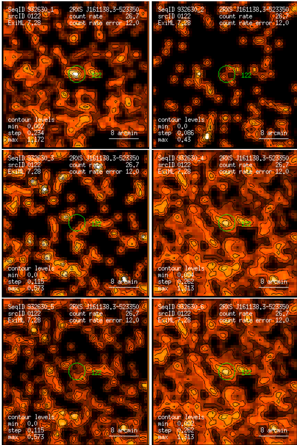
Figure 122: RASS 932630: detection 0122: band rate images, Gaussian filter: (1) PSPC channels 11 – 41, (2) 52 – 90, (3) 91 – 201, (4) 11 – 235, (5) 52 – 201, (6) 11 – 201. Broad band rates in counts/ks. Band rate contour levels in counts/ks/arcmin 2 .
