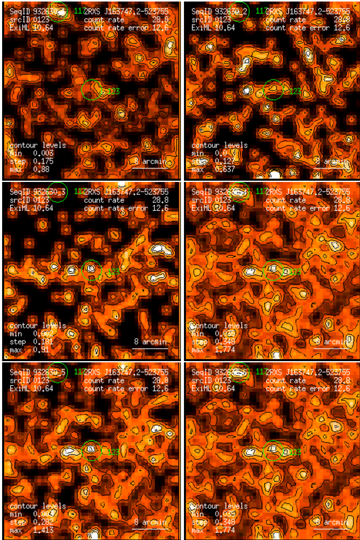
Figure 123: RASS 932630: detection 0123: band rate images, Gaussian filter: (1) PSPC channels 11 – 41, (2) 52 – 90, (3) 91 – 201, (4) 11 – 235, (5) 52 – 201, (6) 11 – 201. Broad band rates in counts/ks. Band rate contour levels in counts/ks/arcmin 2 .
