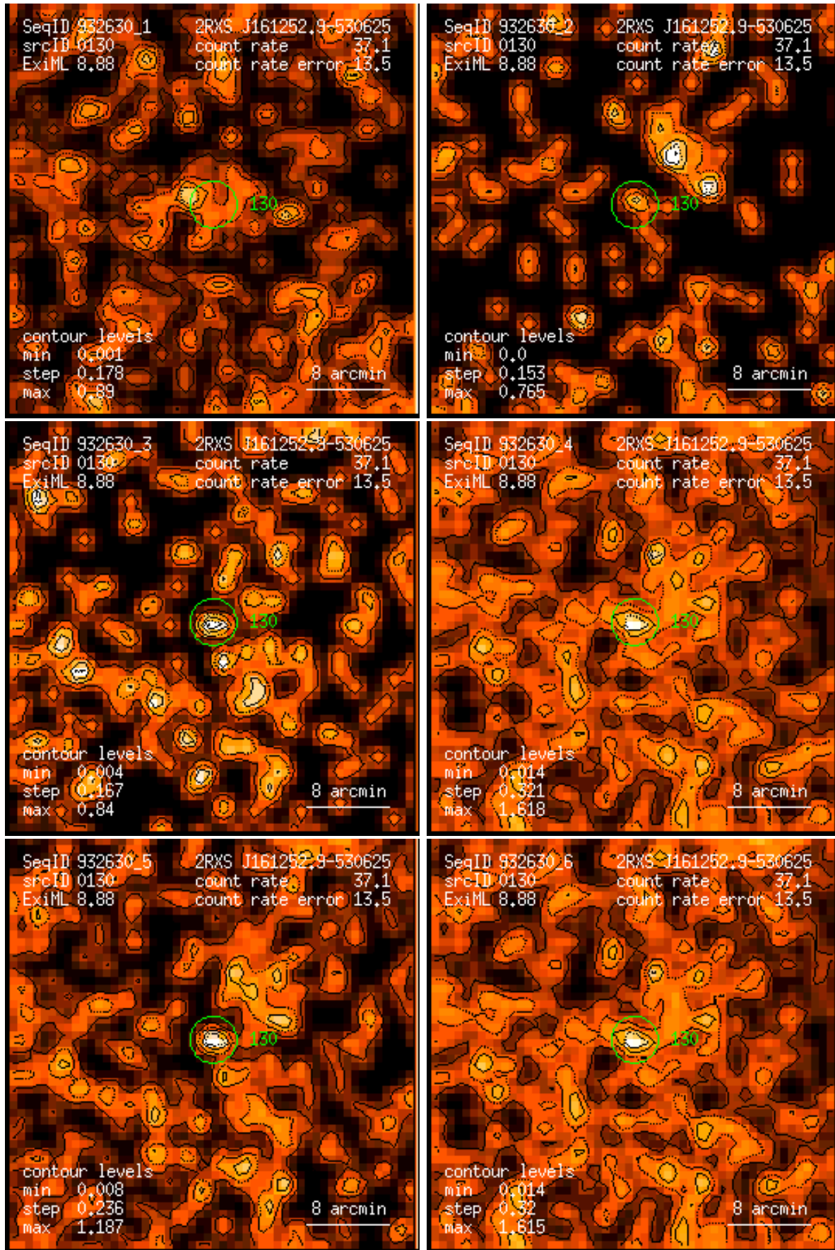
Figure 130: RASS 932630: detection 0130: band rate images, Gaussian filter: (1) PSPC channels 11 – 41, (2) 52 – 90, (3) 91 – 201, (4) 11 – 235, (5) 52 – 201, (6) 11 – 201. Broad band rates in counts/ks. Band rate contour levels in counts/ks/arcmin 2 .
