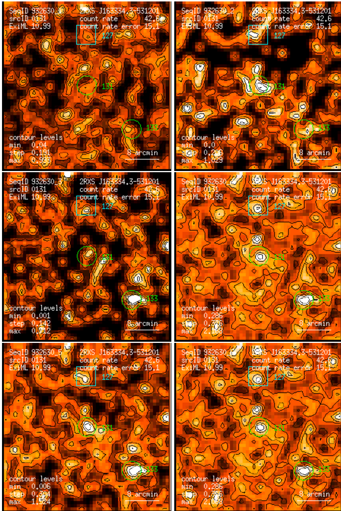
Figure 131: RASS 932630: detection 0131: band rate images, Gaussian filter: (1) PSPC channels 11 – 41, (2) 52 – 90, (3) 91 – 201, (4) 11 – 235, (5) 52 – 201, (6) 11 – 201. Broad band rates in counts/ks. Band rate contour levels in counts/ks/arcmin 2 .
