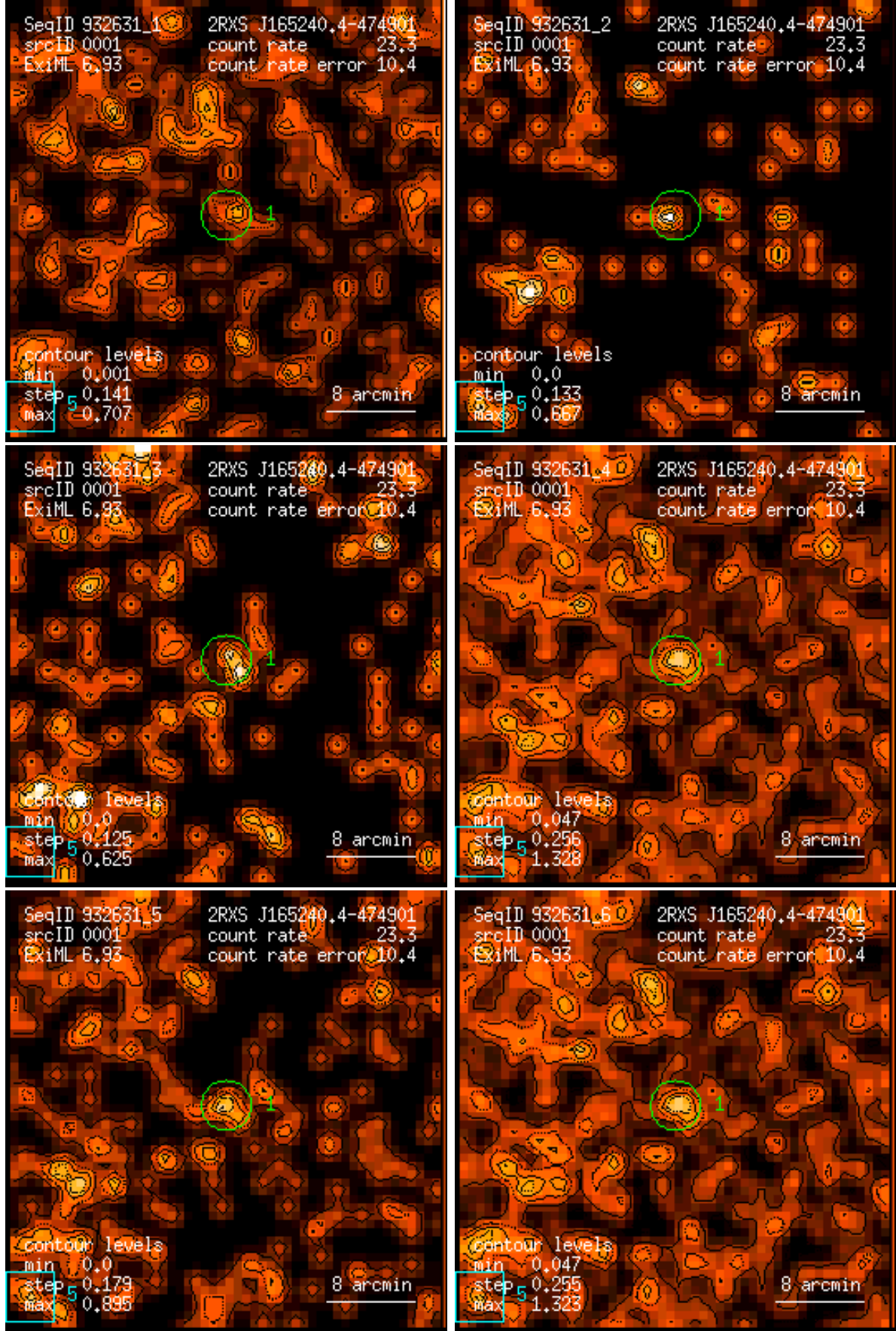
Figure 1: RASS 932631: detection 0001: band rate images, Gaussian filter: (1) PSPC channels 11 – 41, (2) 52 – 90, (3) 91 – 201, (4) 11 – 235, (5) 52 – 201, (6) 11 – 201. Broad band rates in counts/ks. Band rate contour levels in counts/ks/arcmin 2 .
