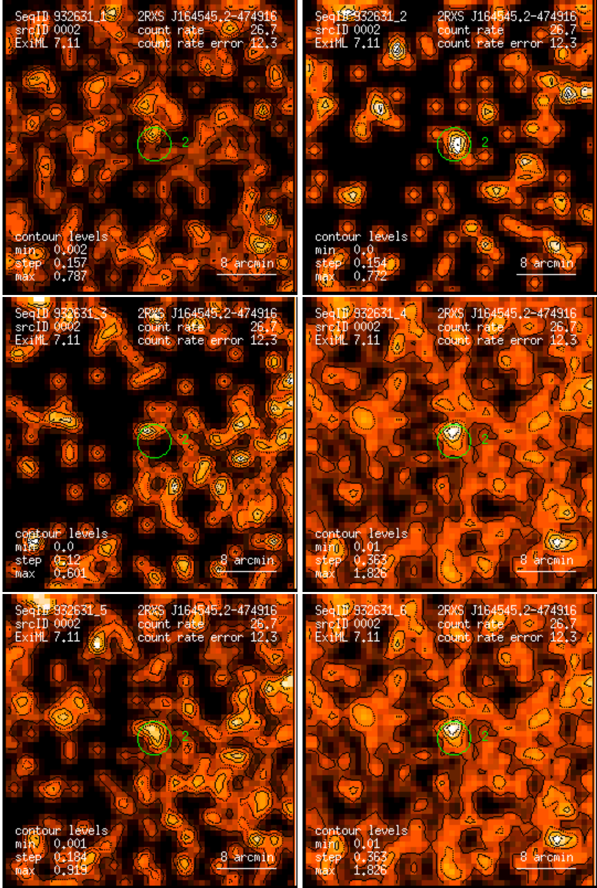
Figure 2: RASS 932631: detection 0002: band rate images, Gaussian filter: (1) PSPC channels 11 – 41, (2) 52 – 90, (3) 91 – 201, (4) 11 – 235, (5) 52 – 201, (6) 11 – 201. Broad band rates in counts/ks. Band rate contour levels in counts/ks/arcmin 2 .
