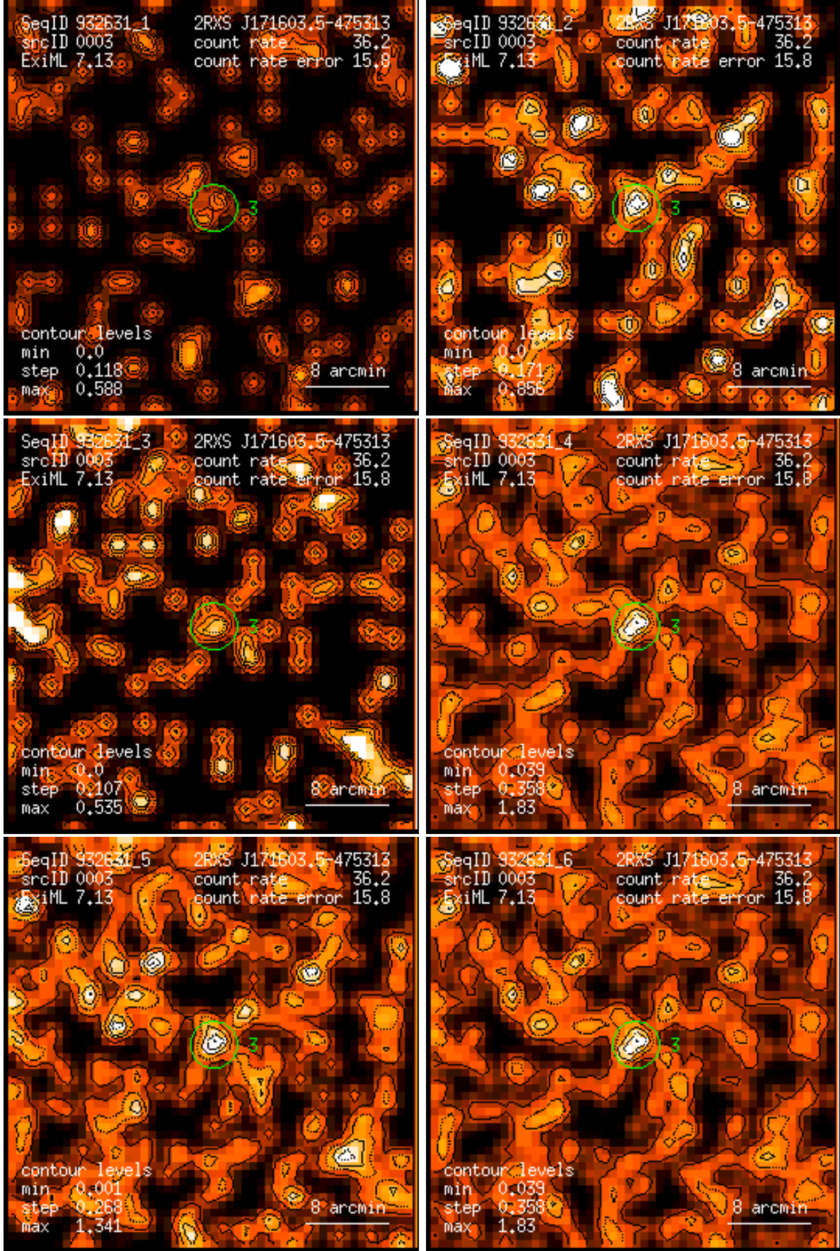
Figure 3: RASS 932631: detection 0003: band rate images, Gaussian filter: (1) PSPC channels 11 – 41, (2) 52 – 90, (3) 91 – 201, (4) 11 – 235, (5) 52 – 201, (6) 11 – 201. Broad band rates in counts/ks. Band rate contour levels in counts/ks/arcmin 2 .
