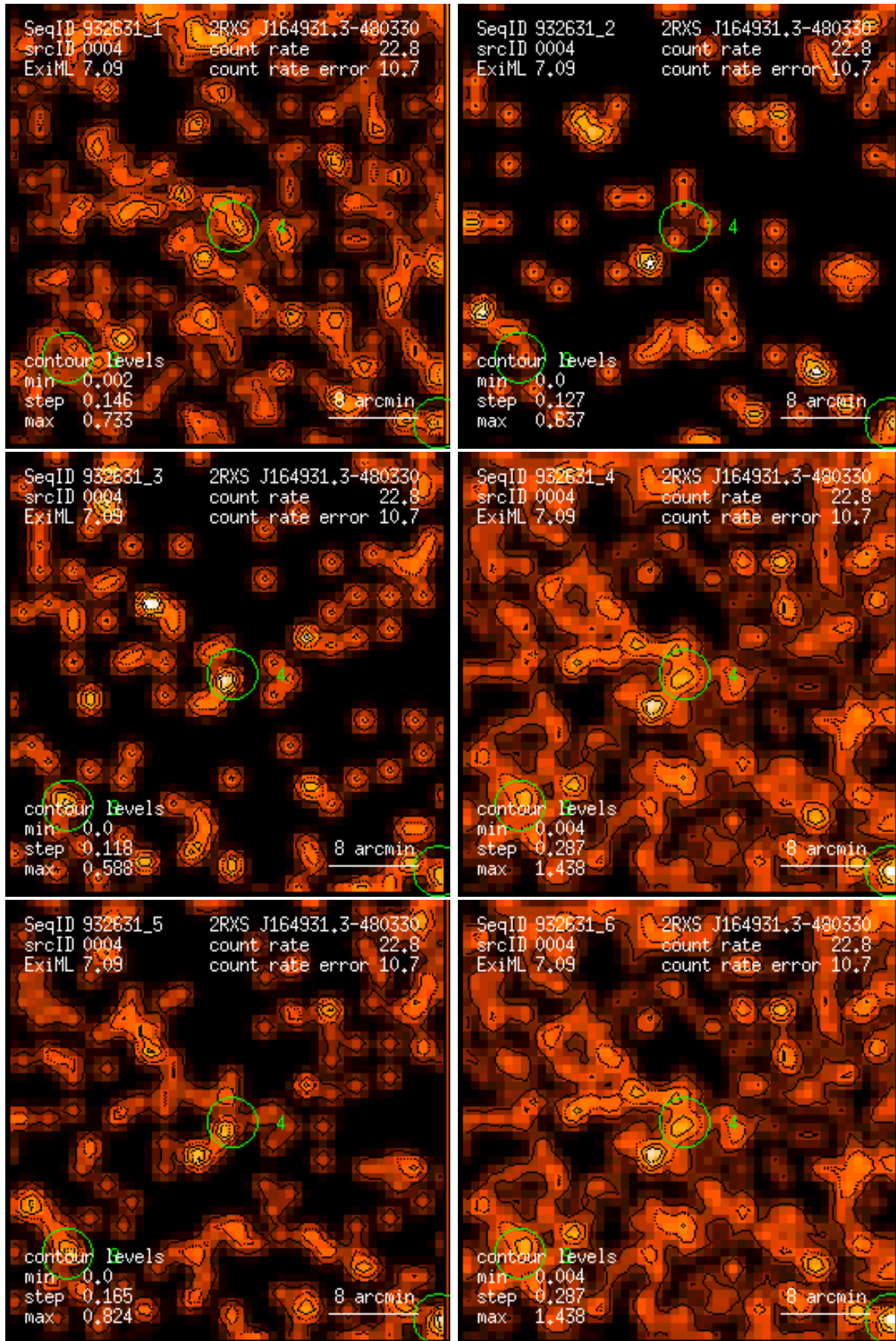
Figure 4: RASS 932631: detection 0004: band rate images, Gaussian filter: (1) PSPC channels 11 – 41, (2) 52 – 90, (3) 91 – 201, (4) 11 – 235, (5) 52 – 201, (6) 11 – 201. Broad band rates in counts/ks. Band rate contour levels in counts/ks/arcmin 2 .
