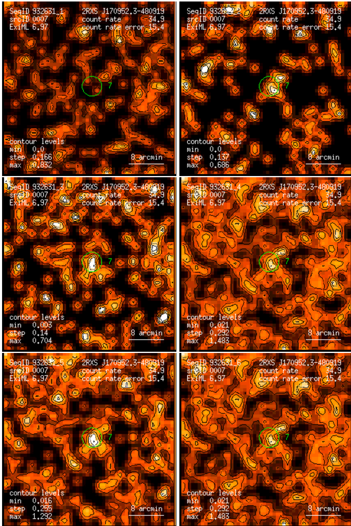
Figure 7: RASS 932631: detection 0007: band rate images, Gaussian filter: (1) PSPC channels 11 – 41, (2) 52 – 90, (3) 91 – 201, (4) 11 – 235, (5) 52 – 201, (6) 11 – 201. Broad band rates in counts/ks. Band rate contour levels in counts/ks/arcmin 2 .
