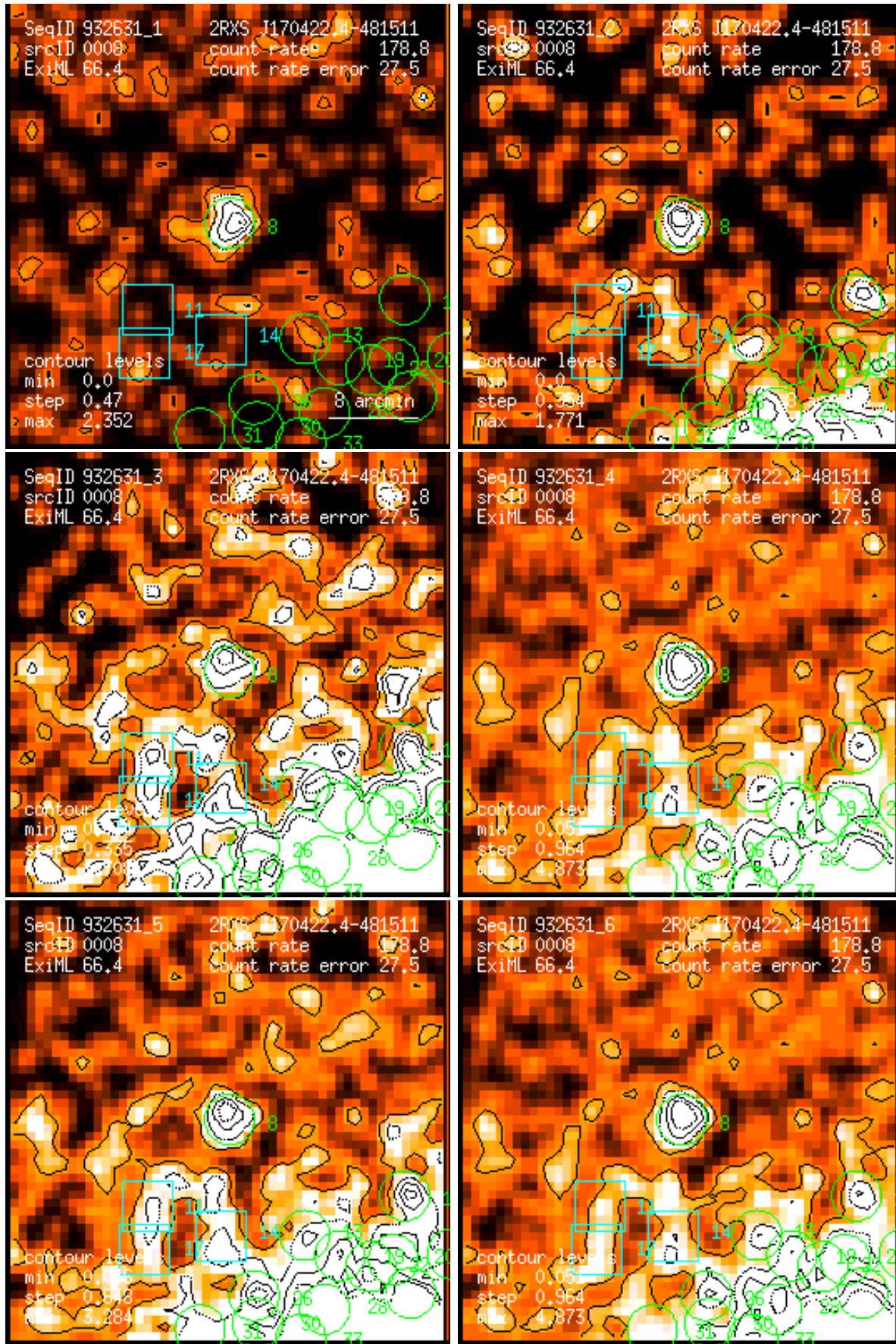
Figure 8: RASS 932631: detection 0008: band rate images, Gaussian filter: (1) PSPC channels 11 – 41, (2) 52 – 90, (3) 91 – 201, (4) 11 – 235, (5) 52 – 201, (6) 11 – 201. Broad band rates in counts/ks. Band rate contour levels in counts/ks/arcmin 2 .
