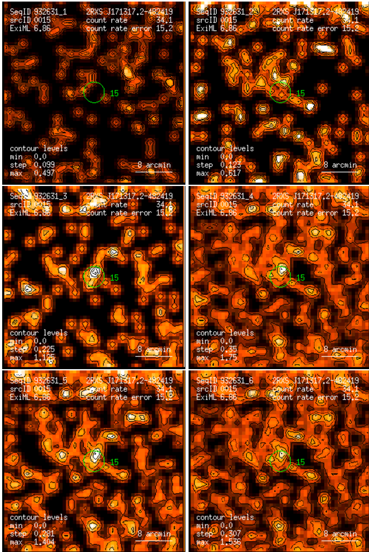
Figure 15: RASS 932631: detection 0015: band rate images, Gaussian filter: (1) PSPC channels 11 – 41, (2) 52 – 90, (3) 91 – 201, (4) 11 – 235, (5) 52 – 201, (6) 11 – 201. Broad band rates in counts/ks. Band rate contour levels in counts/ks/arcmin 2 .
