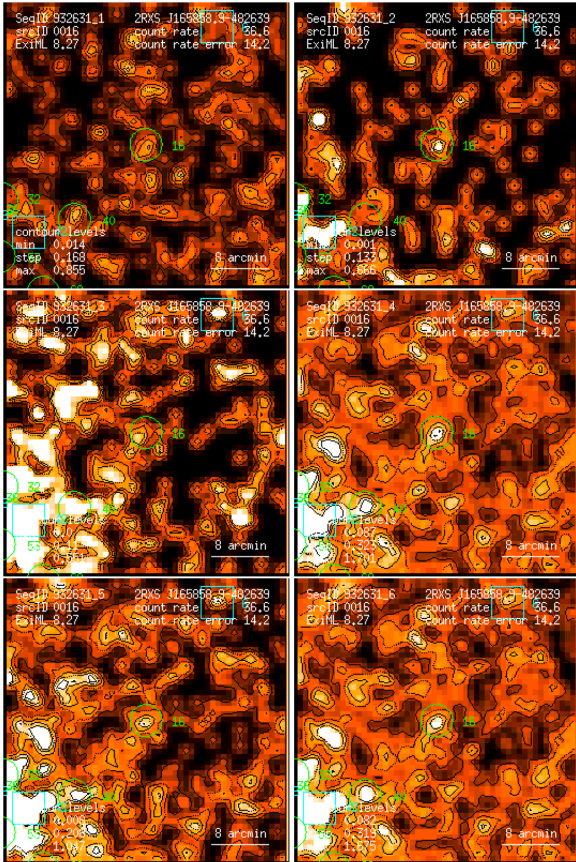
Figure 16: RASS 932631: detection 0016: band rate images, Gaussian filter: (1) PSPC channels 11 – 41, (2) 52 – 90, (3) 91 – 201, (4) 11 – 235, (5) 52 – 201, (6) 11 – 201. Broad band rates in counts/ks. Band rate contour levels in counts/ks/arcmin 2 .
