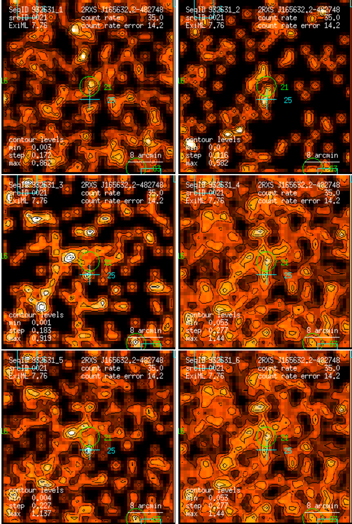
Figure 21: RASS 932631: detection 0021: band rate images, Gaussian filter: (1) PSPC channels 11 – 41, (2) 52 – 90, (3) 91 – 201, (4) 11 – 235, (5) 52 – 201, (6) 11 – 201. Broad band rates in counts/ks. Band rate contour levels in counts/ks/arcmin 2 .
