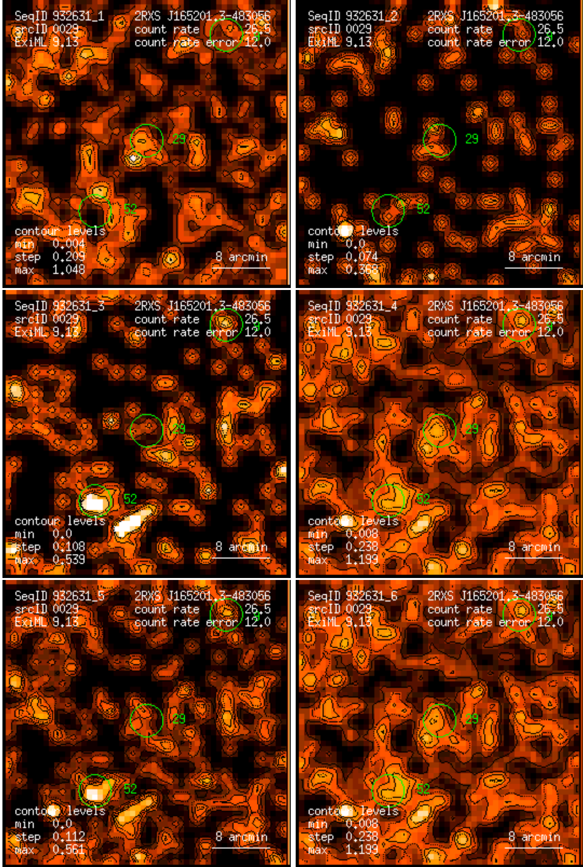
Figure 29: RASS 932631: detection 0029: band rate images, Gaussian filter: (1) PSPC channels 11 – 41, (2) 52 – 90, (3) 91 – 201, (4) 11 – 235, (5) 52 – 201, (6) 11 – 201. Broad band rates in counts/ks. Band rate contour levels in counts/ks/arcmin 2 .
