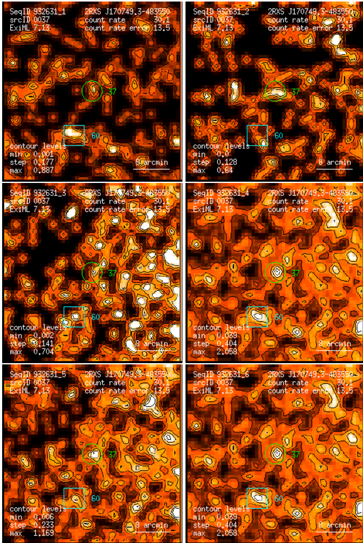
Figure 37: RASS 932631: detection 0037: band rate images, Gaussian filter: (1) PSPC channels 11 – 41, (2) 52 – 90, (3) 91 – 201, (4) 11 – 235, (5) 52 – 201, (6) 11 – 201. Broad band rates in counts/ks. Band rate contour levels in counts/ks/arcmin 2 .
