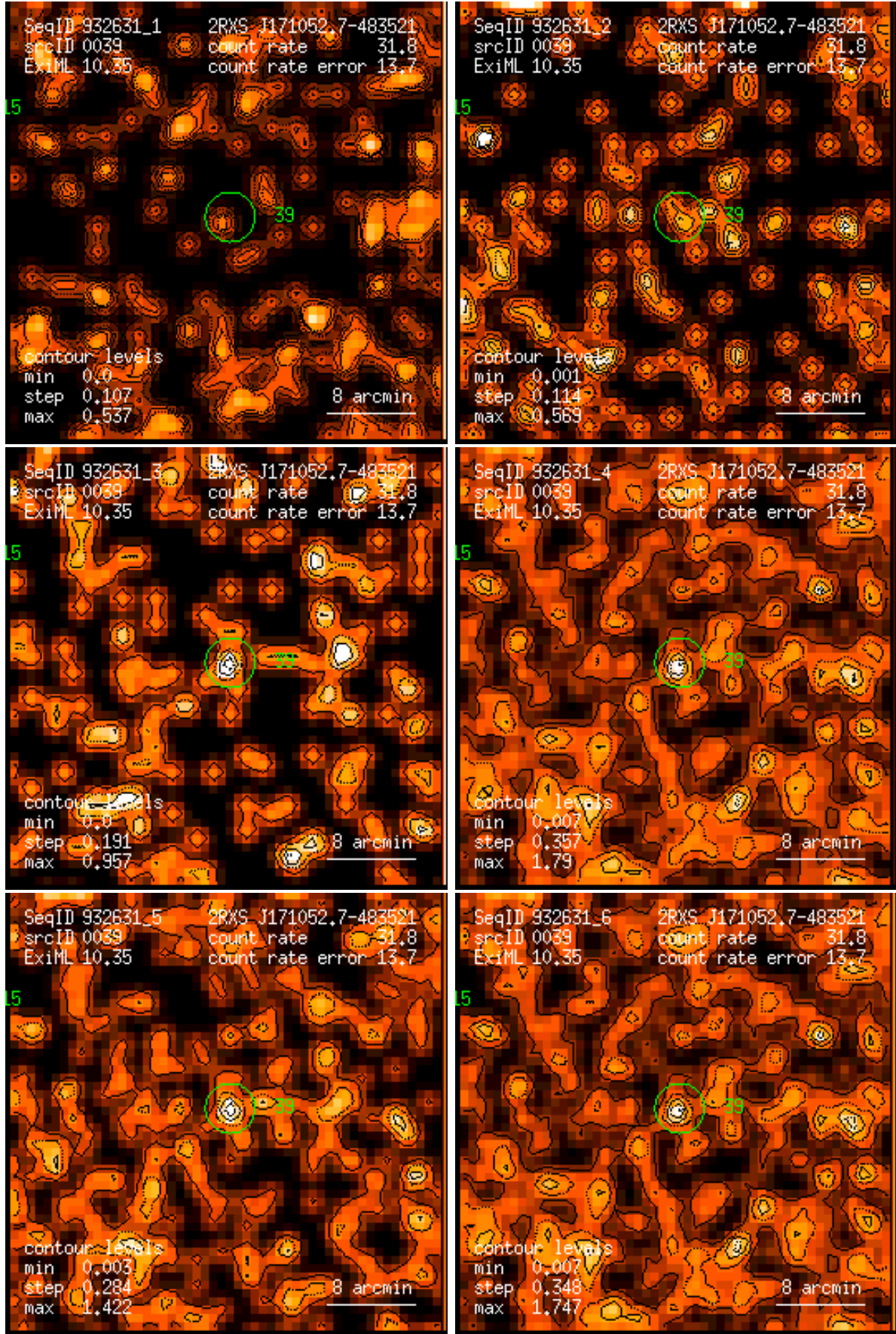
Figure 39: RASS 932631: detection 0039: band rate images, Gaussian filter: (1) PSPC channels 11 – 41, (2) 52 – 90, (3) 91 – 201, (4) 11 – 235, (5) 52 – 201, (6) 11 – 201. Broad band rates in counts/ks. Band rate contour levels in counts/ks/arcmin 2 .
