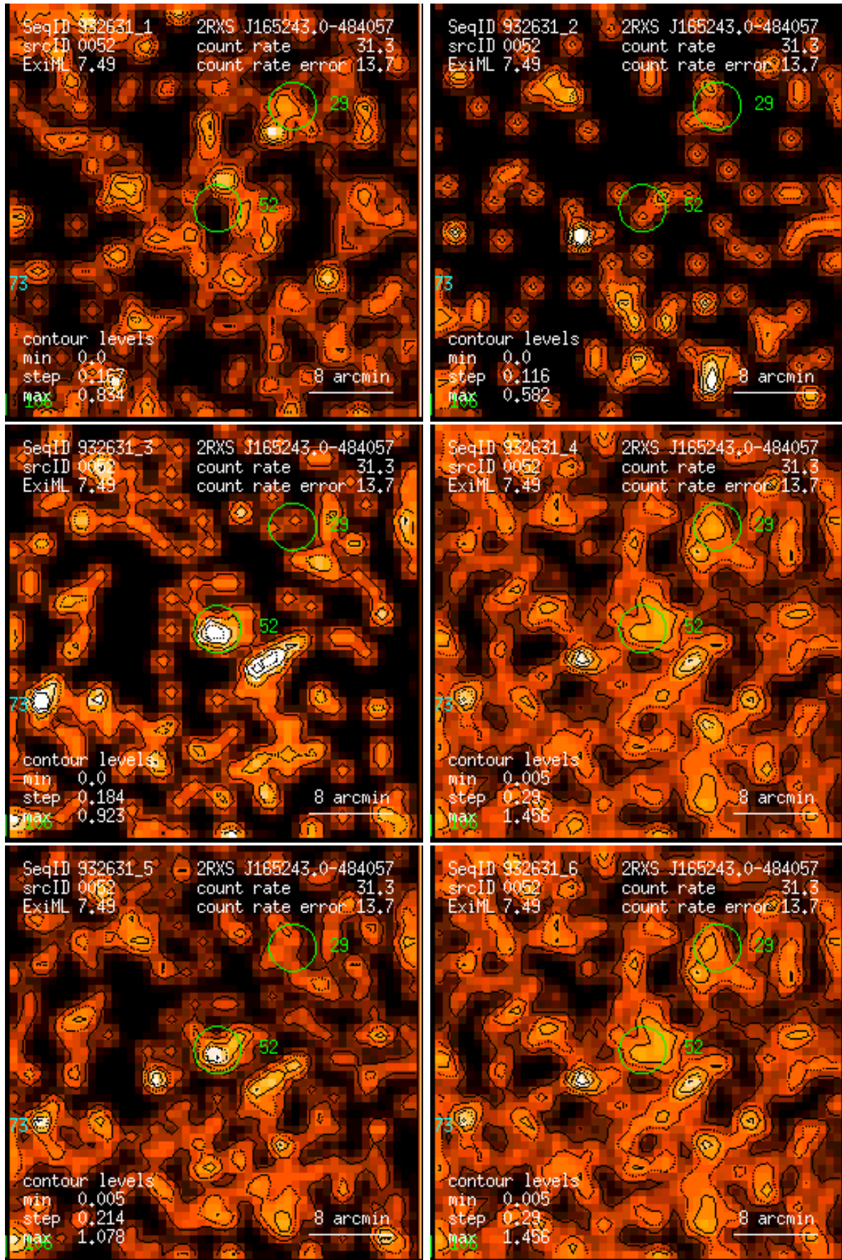
Figure 52: RASS 932631: detection 0052: band rate images, Gaussian filter: (1) PSPC channels 11 – 41, (2) 52 – 90, (3) 91 – 201, (4) 11 – 235, (5) 52 – 201, (6) 11 – 201. Broad band rates in counts/ks. Band rate contour levels in counts/ks/arcmin 2 .
