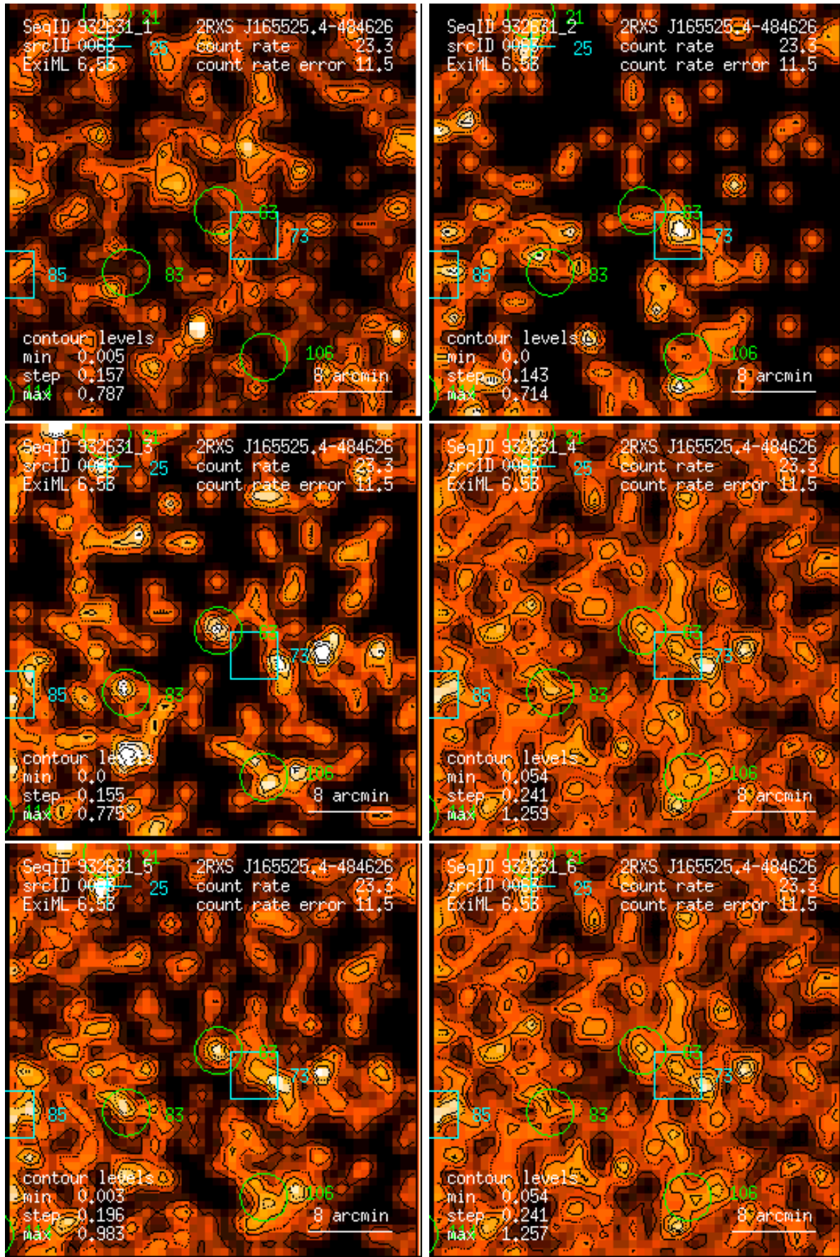
Figure 63: RASS 932631: detection 0063: band rate images, Gaussian filter: (1) PSPC channels 11 – 41, (2) 52 – 90, (3) 91 – 201, (4) 11 – 235, (5) 52 – 201, (6) 11 – 201. Broad band rates in counts/ks. Band rate contour levels in counts/ks/arcmin 2 .
