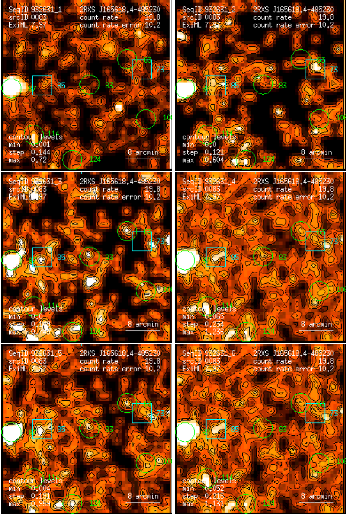
Figure 83: RASS 932631: detection 0083: band rate images, Gaussian filter: (1) PSPC channels 11 – 41, (2) 52 – 90, (3) 91 – 201, (4) 11 – 235, (5) 52 – 201, (6) 11 – 201. Broad band rates in counts/ks. Band rate contour levels in counts/ks/arcmin 2 .
