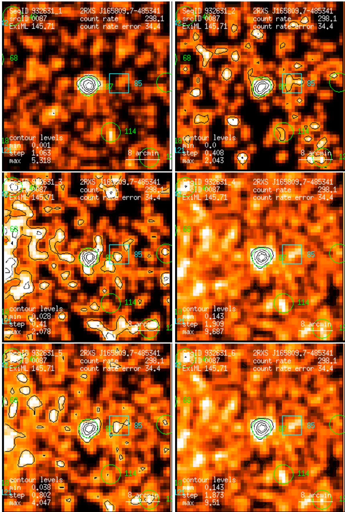
Figure 87: RASS 932631: detection 0087: band rate images, Gaussian filter: (1) PSPC channels 11 – 41, (2) 52 – 90, (3) 91 – 201, (4) 11 – 235, (5) 52 – 201, (6) 11 – 201. Broad band rates in counts/ks. Band rate contour levels in counts/ks/arcmin 2 .
