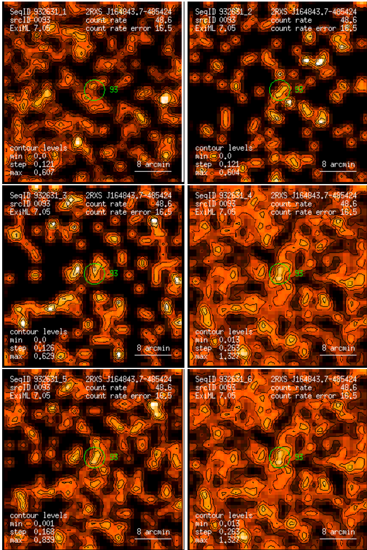
Figure 93: RASS 932631: detection 0093: band rate images, Gaussian filter: (1) PSPC channels 11 – 41, (2) 52 – 90, (3) 91 – 201, (4) 11 – 235, (5) 52 – 201, (6) 11 – 201. Broad band rates in counts/ks. Band rate contour levels in counts/ks/arcmin 2 .
