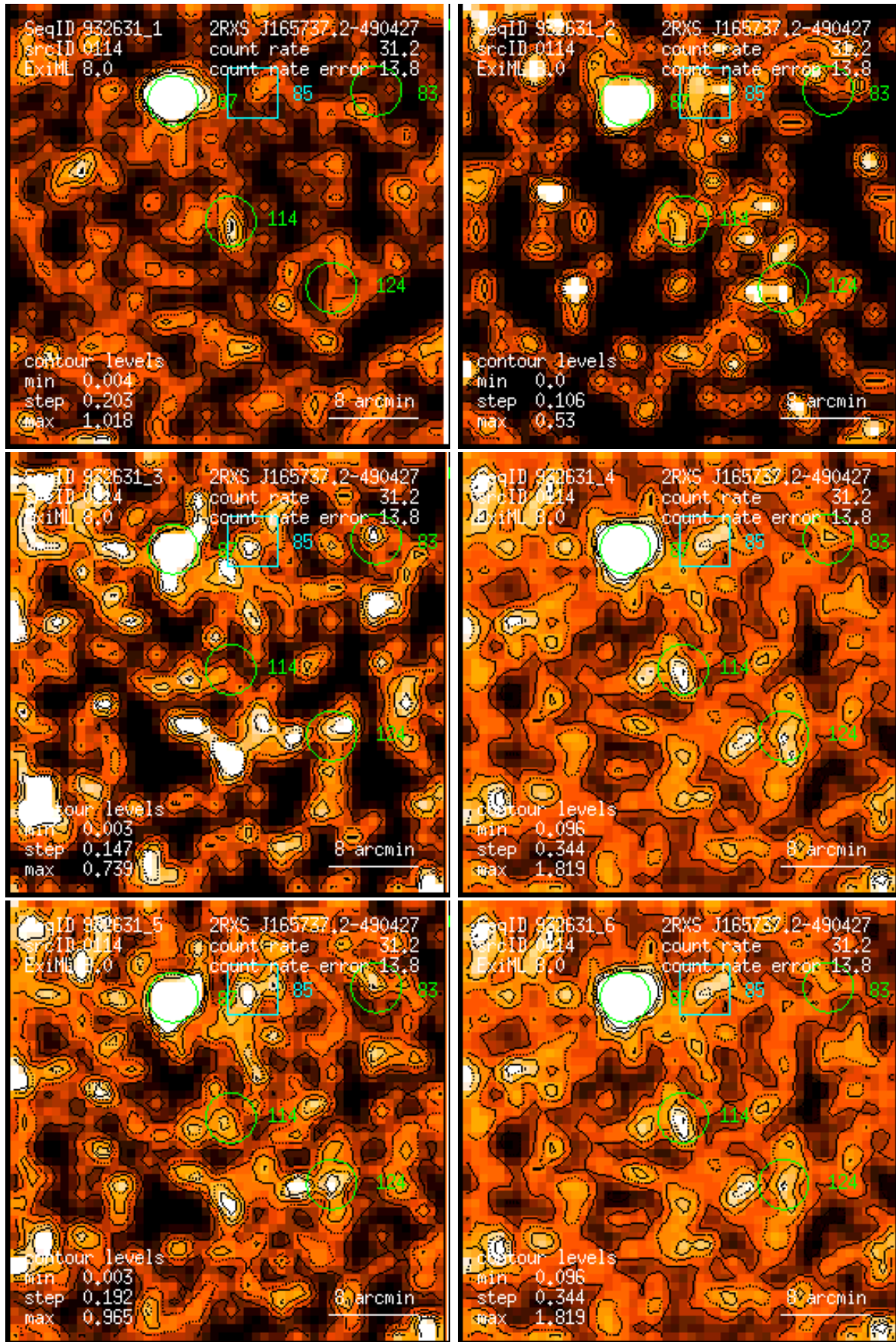
Figure 114: RASS 932631: detection 0114: band rate images, Gaussian filter: (1) PSPC channels 11 – 41, (2) 52 – 90, (3) 91 – 201, (4) 11 – 235, (5) 52 – 201, (6) 11 – 201. Broad band rates in counts/ks. Band rate contour levels in counts/ks/arcmin 2 .
