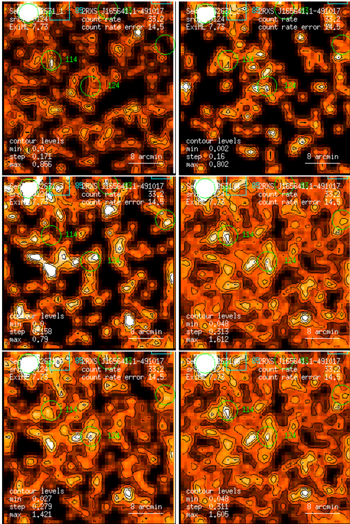
Figure 124: RASS 932631: detection 0124: band rate images, Gaussian filter: (1) PSPC channels 11 – 41, (2) 52 – 90, (3) 91 – 201, (4) 11 – 235, (5) 52 – 201, (6) 11 – 201. Broad band rates in counts/ks. Band rate contour levels in counts/ks/arcmin 2 .
